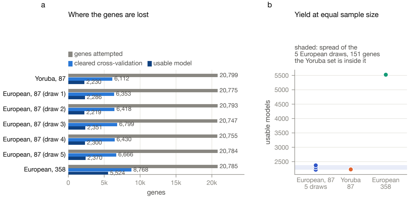
Fig. 6. Model yield. (a) For each training set, the genes attempted, those clearing the cross-validation criteria, and those retaining a usable model after the final fit. (b) Usable models per set. The shaded band is the spread between the European draws of 87, against which the Yoruba count can be read directly.
