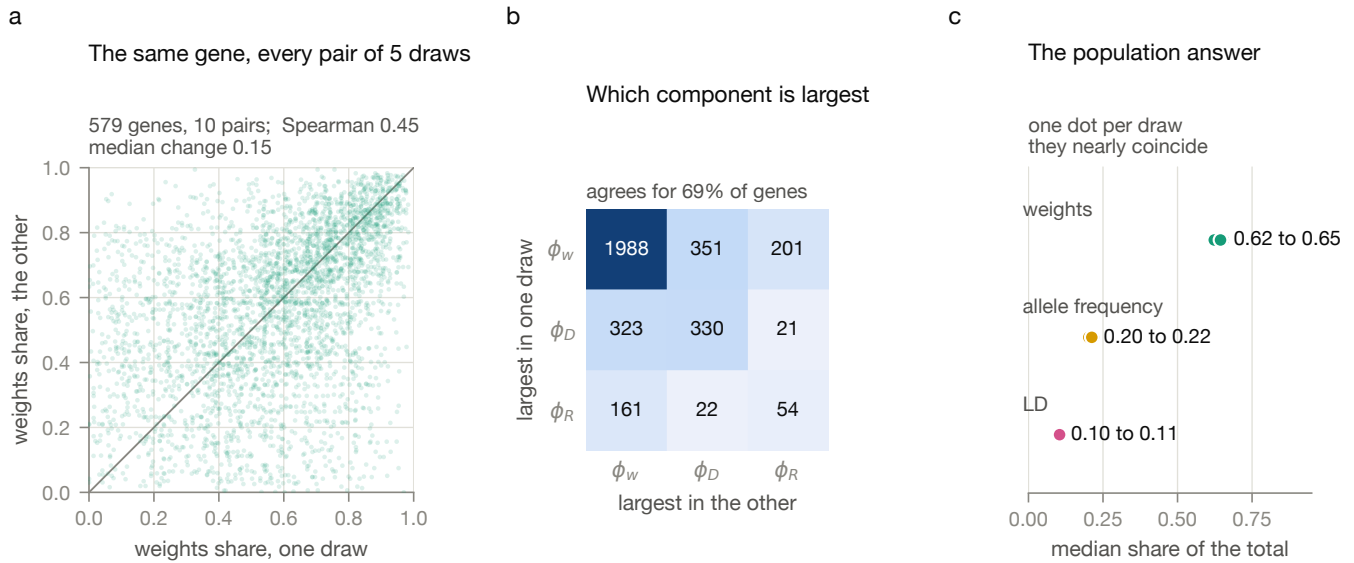
Fig. 13. How much the answer depends on the draw. The decomposition is run against the same Yoruba sample with five independent random draws of 87 European individuals, and panels (a) and (b) pool all ten pairs of draws. (a) Each gene's weights share in one draw against another. (b) Which component is largest for a gene, one draw against another. (c) The median share of each component, one dot per draw.
