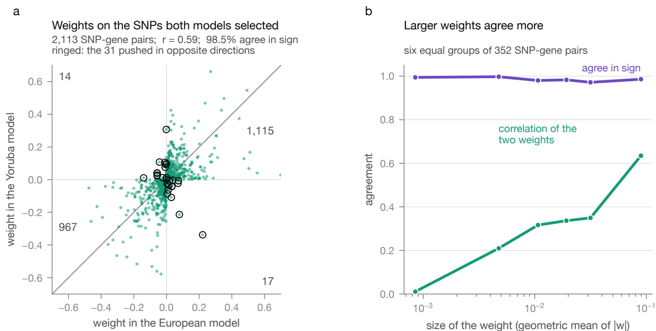
Fig. 7. Agreement on shared predictors. (a) Every SNP selected by both the European and the Yoruba model for the same gene, placed by the weight each model gave it. The line marks equal weights. Ringed points are the 31 SNPs the two models push in opposite directions, and the corner numbers count the SNPs in each quadrant. (b) Sign agreement and the correlation of the two weights within six equal groups of SNPs, ordered by the size of the weight.
