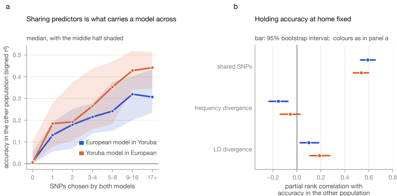
Fig. 15. What carries a model across. (a) Cross-population accuracy against the number of SNPs both models selected for the same gene, in both directions, as a median with the middle half shaded. (b) Partial rank correlation of each predictor with cross-population accuracy, holding the model's accuracy at home fixed, with 95% bootstrap intervals. Colours are as in panel (a).
