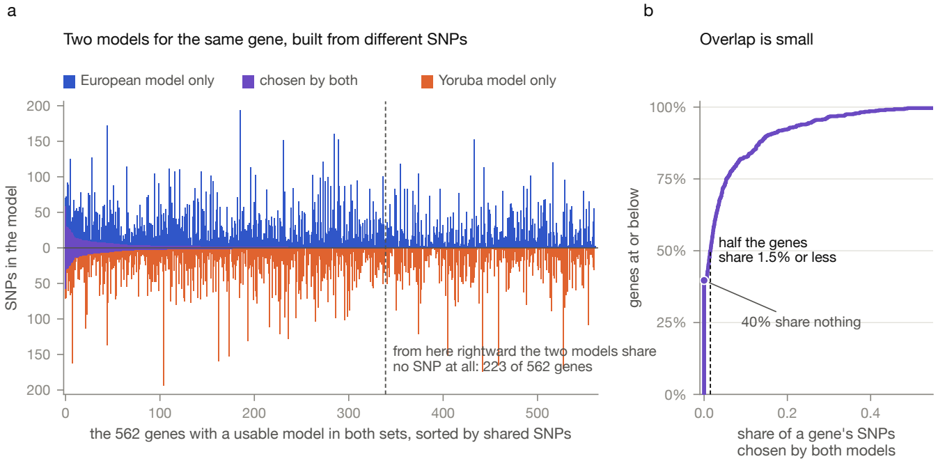
Fig. 8. The two models are built from different SNPs. (a) One column per gene with a usable model in both sets, sorted by the number of SNPs the two models share. The shared SNPs form the band straddling the axis, the SNPs only the European model chose rise above it, and the SNPs only the Yoruba model chose fall below. To the right of the dashed line the two models share no SNP at all. (b) The share of a gene's SNPs chosen by both models, read cumulatively.
