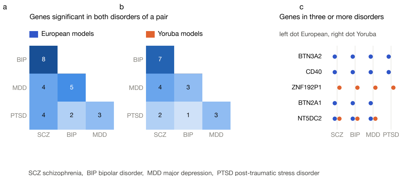
Fig. 20. Genes shared across disorders. (a, b) The number of genes reaching Bonferroni significance for both disorders of each pair, for the European and the Yoruba model set. (c) Every gene significant in three or more disorders, with a dot per model set that found it.
