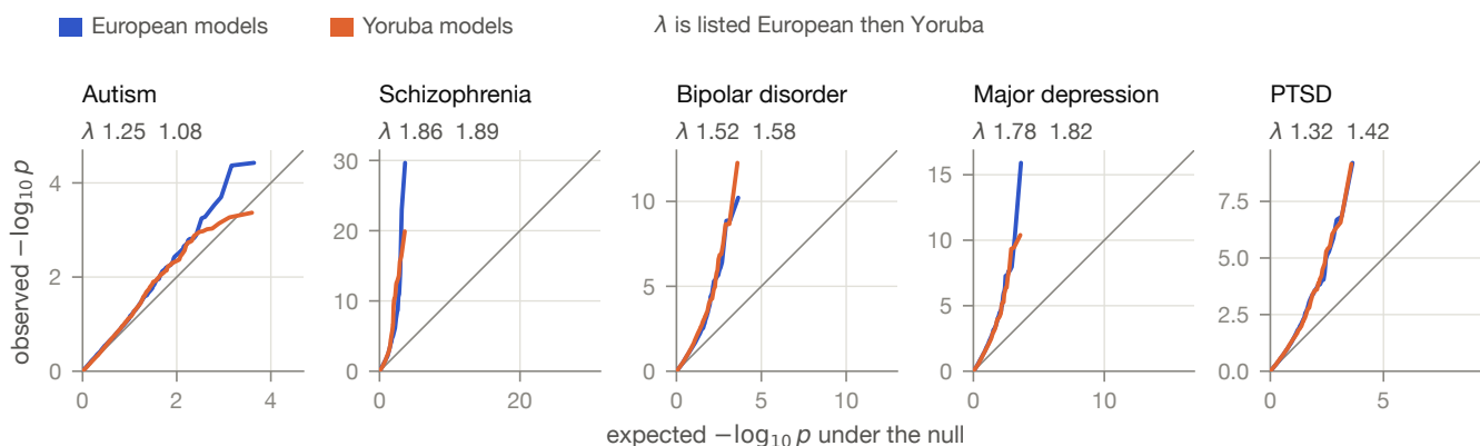
Fig. 18. Calibration of the association tests. Observed against expected -\log_{10} p under the null for each trait, with the European and Yoruba model sets drawn together and the null diagonal marked. Genomic inflation \lambda is printed per panel, European then Yoruba. Each panel carries its own scale because the observed range differs by almost an order of magnitude between traits.
