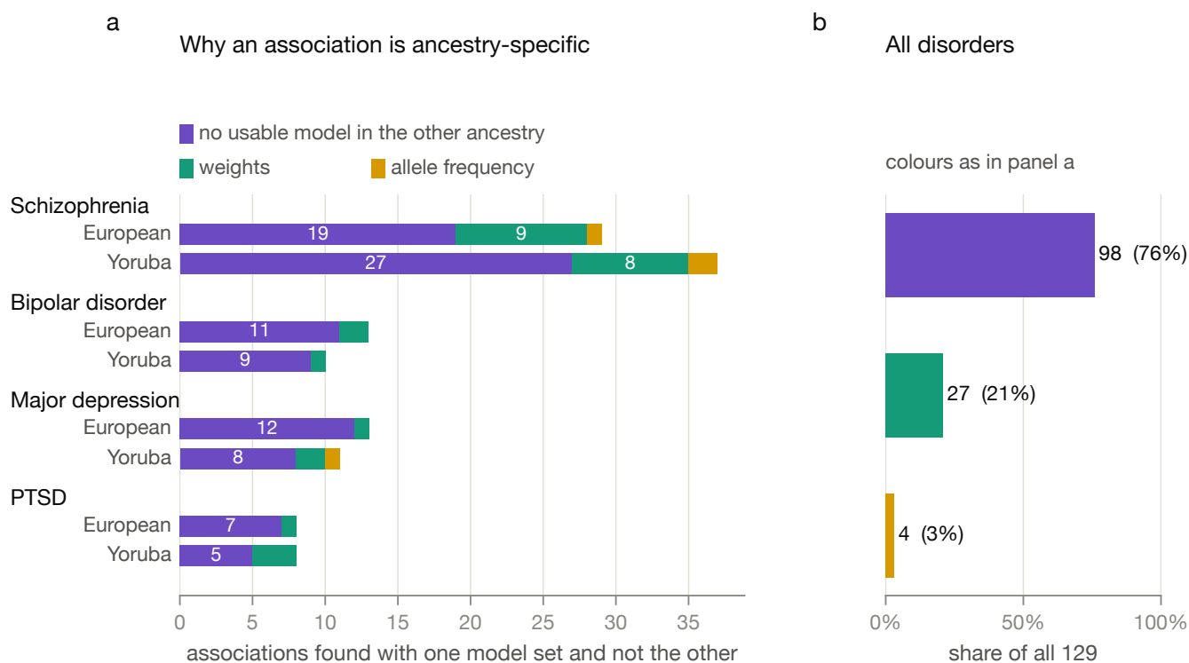
Fig. 19. Why an association is ancestry-specific. (a) For each disorder and each model set, the associations found with that set and not the other, split by whether the other ancestry produced a usable model for the gene at all and, where it did, by the largest component of the decomposition. (b) The same 129 associations pooled across disorders.
