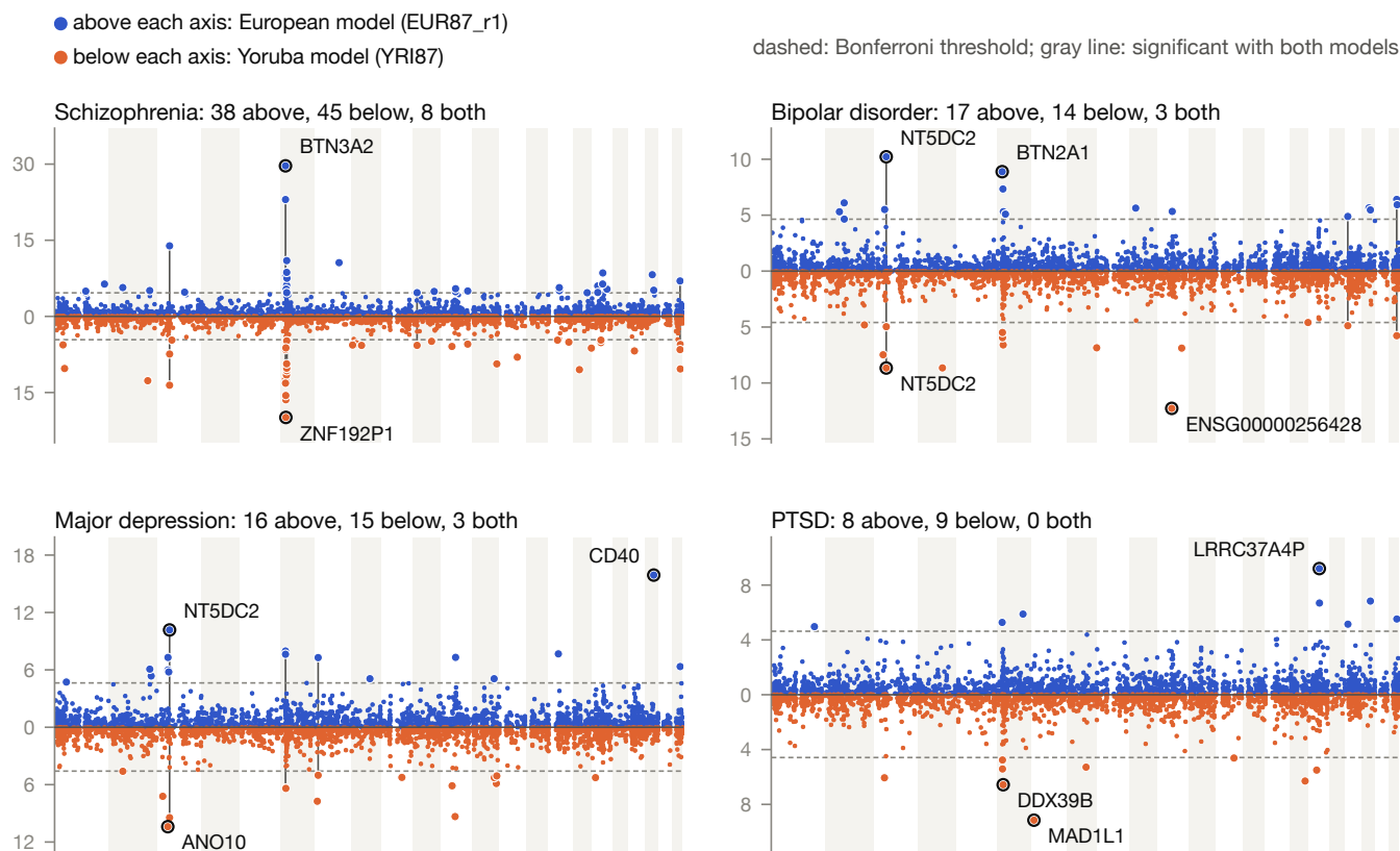
Fig. 17. Summary-statistic TWAS for schizophrenia, bipolar disorder, major depression and post-traumatic stress disorder, with the European model set above each axis and the Yoruba model set below. Gray vertical lines connect a gene significant with both model sets.
