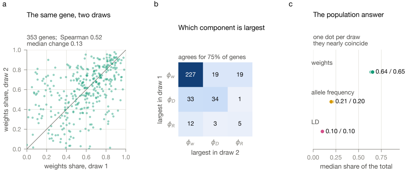
Fig. 12. How much the answer depends on the draw. The decomposition is run twice against the same Yoruba sample, using two independent random draws of 87 European individuals. (a) Each gene's weights share in one draw against the other. (b) Which component is largest for a gene, one draw against the other. (c) The median share of each component, one dot per draw.
