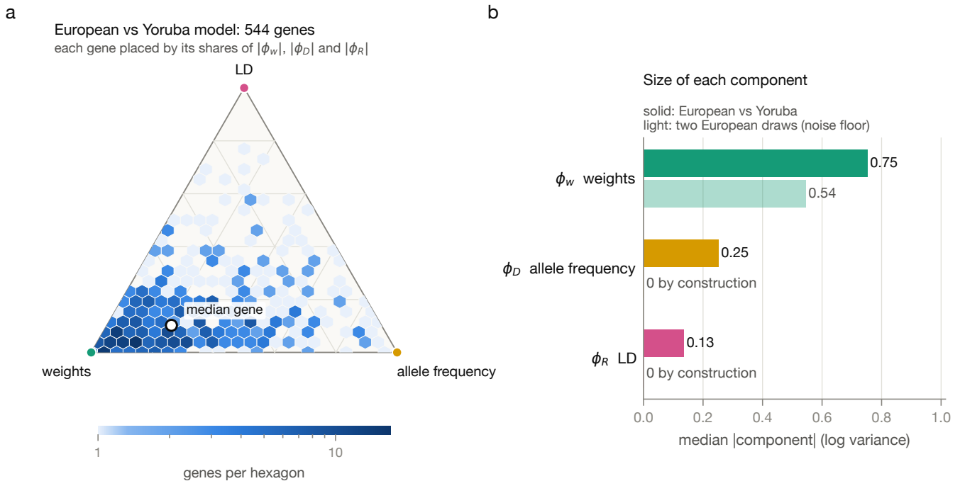
Fig. 9. Where the disagreement between two models comes from. (a) Each gene placed by its shares of |\phi_w| , |\phi_D| and |\phi_R| , with density on a logarithmic scale and the median gene ringed. (b) Median absolute component between the European and Yoruba models (solid) beside the within-ancestry noise floor from two independent European draws (light), where the frequency and LD components are exactly zero by construction.
