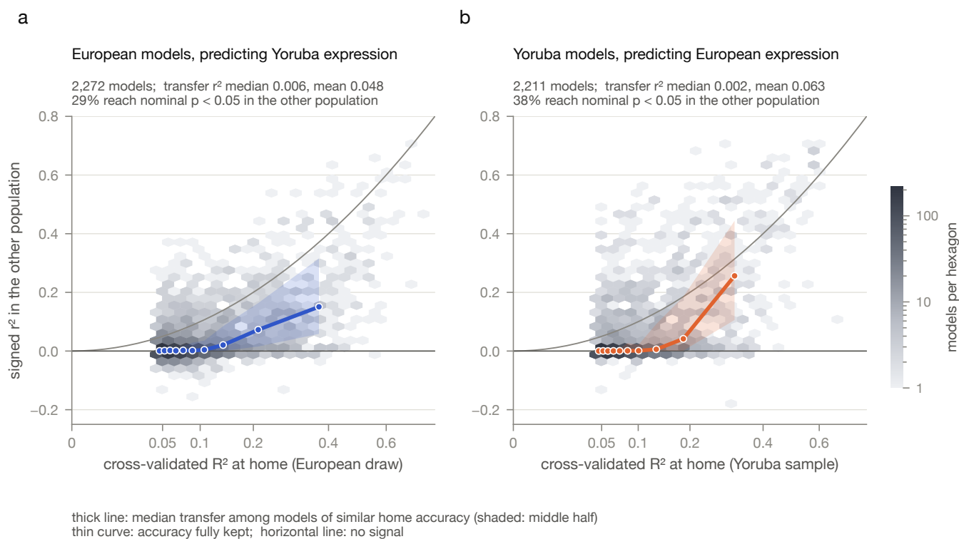
Fig. 14. How much accuracy survives a crossing. (a) Every usable European model applied to the Yoruba individuals and (b) every usable Yoruba model applied to the European individuals, against the model's cross-validated accuracy at home on a square-root axis. The thick line is the median transferred accuracy among models of similar home accuracy, with the middle half shaded. The thin curve marks accuracy fully kept and the horizontal line marks no signal.
