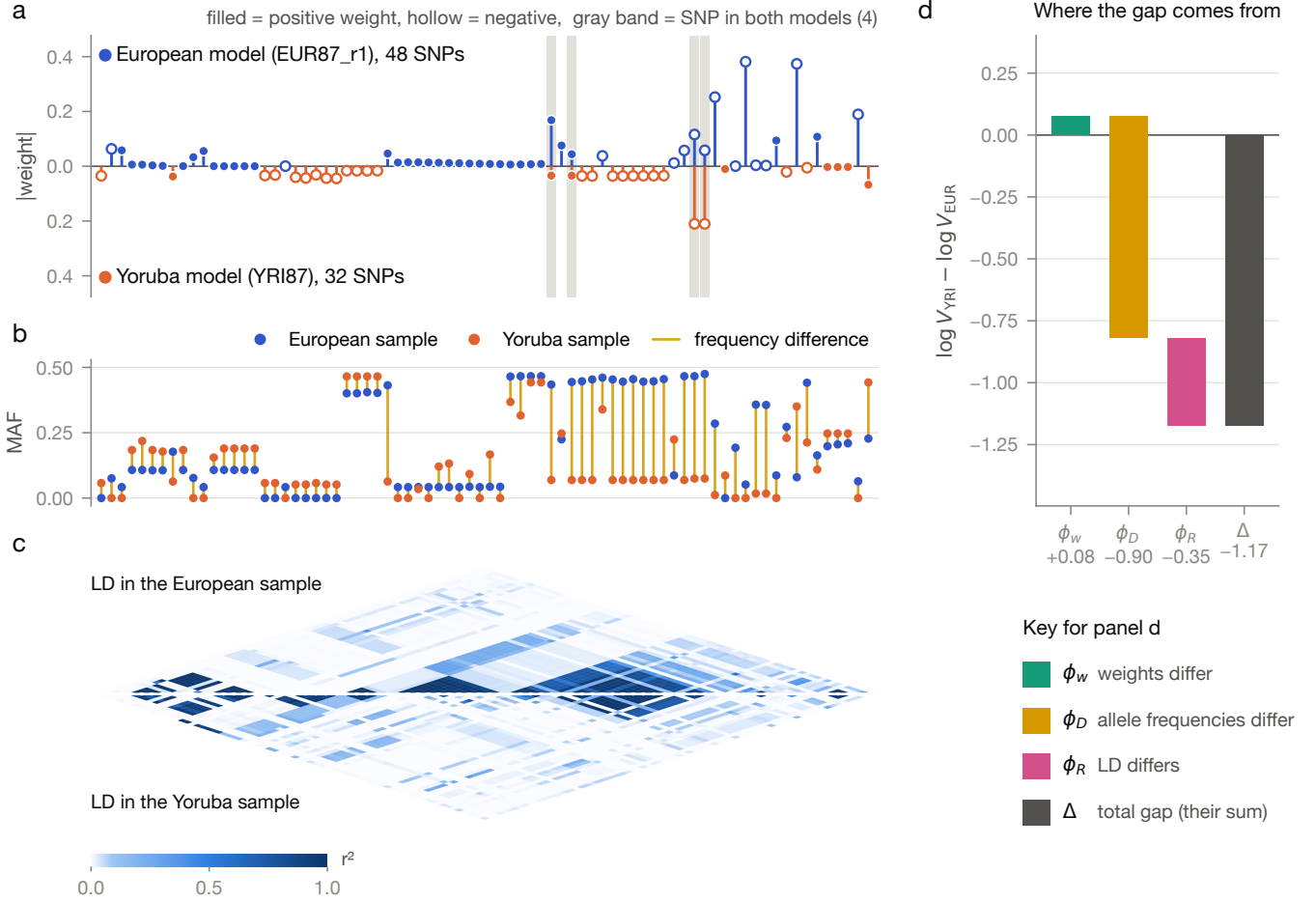
Fig. 11. Anatomy of one disagreement, at DNAJB7. (a) Model weights, European above and Yoruba below, with grey bands marking the four SNPs both models selected. (b) Minor allele frequency of each model SNP in the two samples, joined by a line whose length is the difference. (c) Pairwise r^2 among the same SNPs in each sample. (d) The gap for this gene split into its three components and their sum.
