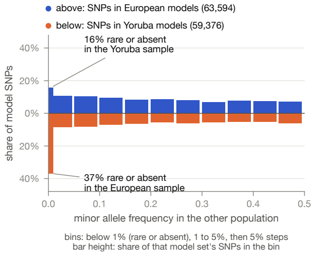
Fig. 13. What each population can see of the other's models. The SNVs selected by usable models, binned by their minor allele frequency in the other population, European models above the axis and Yoruba models below. The leftmost bin holds variants that are rare or absent there.
