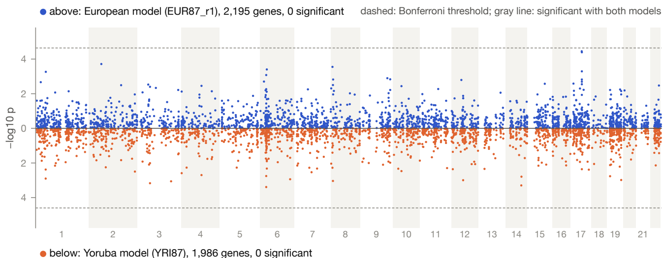
Fig. 16. Summary-statistic TWAS for autism, with the European model set above each axis and the Yoruba model set below. Dashed lines are the Bonferroni threshold for the genes each set could test.
