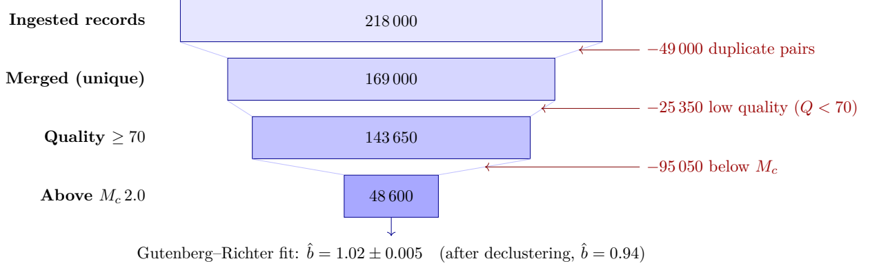
Figure 3: Quantitative event-count flow through the CofC pipeline for the synthetic worked example (Section 6). Bar widths are proportional to the number of events; each stage removes a characterised subset (red) before the Gutenberg–Richter b -value is estimated on the surviving population. All counts are properties of the controlled synthetic inputs, not real New Zealand seismicity.
