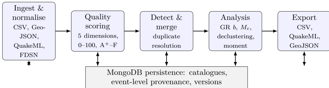
Figure 2: The CofC processing pipeline. Heterogeneous catalogues are ingested and normalised to a canonical schema, quality-scored per event on import (Section 3), merged with configurable duplicate detection (Section 4), analysed in the browser (Section 5), and re-exported in standard formats (Section 6). All stages read and write a MongoDB store that retains catalogues, event-level provenance, and version metadata.
