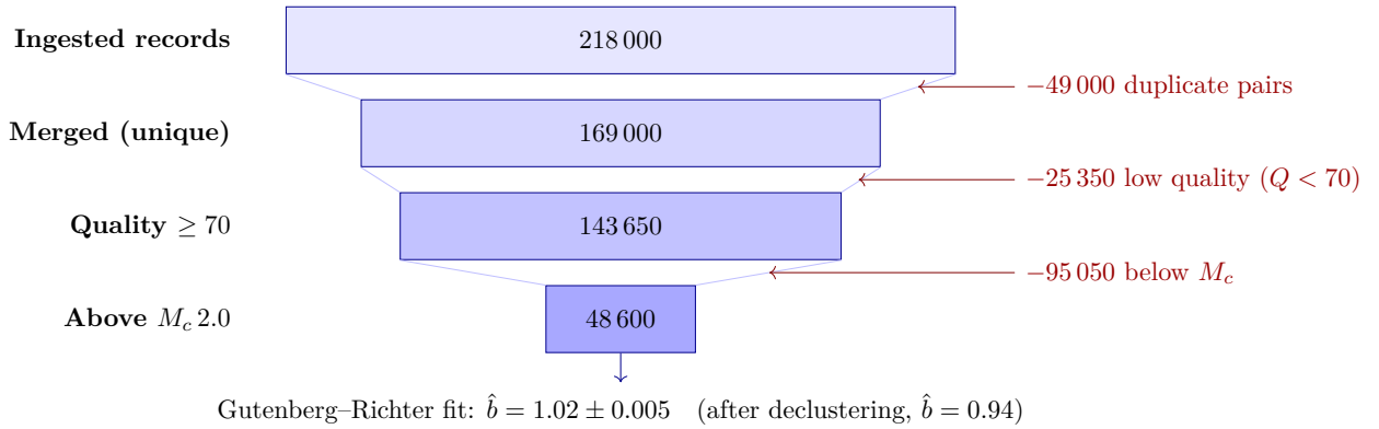
Figure 7: Quantitative event-count flow through the CofC pipeline for the synthetic worked example (Section 7). Bar widths are proportional to the number of events; each stage removes a characterised subset (red) before the Gutenberg–Richter b -value is estimated on the surviving population. All counts are properties of the controlled synthetic inputs, not real New Zealand seismicity.
