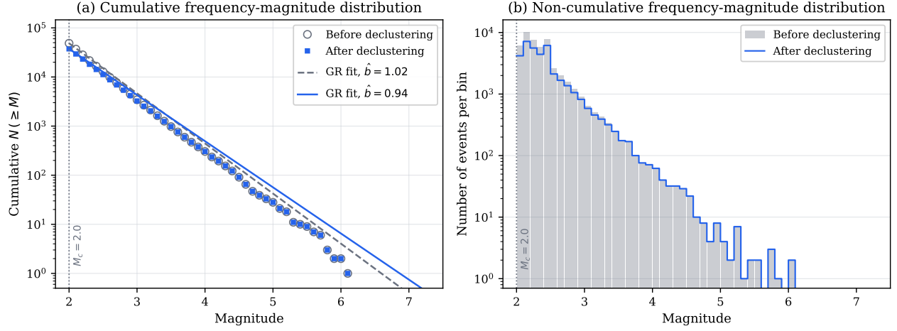
Figure 7: Frequency-magnitude distributions (FMD) for the synthetic New Zealand catalogue before (grey open circles and bars) and after (blue filled squares and step outline) Gardner-Knopoff declustering. (a) Cumulative FMD with maximum-likelihood GR fits (grey dashed line: before; blue solid line: after) above M_c = 2.0 (dotted vertical line); the shallower slope of the declustered fit is the \hat{b} shift quoted below. (b) Non-cumulative FMD showing the excess of small events contributed by aftershock sequences. Declustering removes these clustered small events, shifting \hat{b} from 1.02 \pm 0.005 (before declustering) to 0.94 \pm 0.005 (declustered) and removing 23% of events. Data are synthetic and for illustration only (see Section 7).
