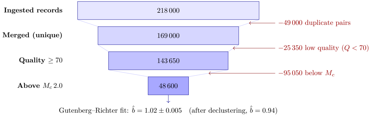
Figure 8: Quantitative event-count flow through the CofC pipeline for the synthetic worked example (Section 7). Bar widths are proportional to the number of events; each stage removes a characterised subset (red) before the Gutenberg-Richter b -value is estimated on the surviving population. All counts are properties of the controlled synthetic inputs, not real New Zealand seismicity.
