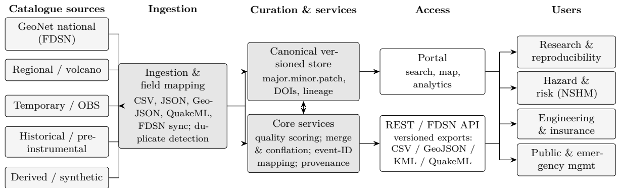
Figure 2: End-to-end architecture of the proposed framework. Heterogeneous catalogue sources are ingested and mapped to a canonical, versioned store; curation services (quality scoring, merge and conflation, event-identifier mapping, and provenance) feed a portal and a programmatic API that serve research, hazard, engineering, and public users. Capabilities identified as implemented in Section 3.1 are exercised end-to-end by the prototype. The figure details the Platform layer; the Registry — the lightweight layer of catalogue submission profiles (Table 3) through which catalogues are first described and discovered — is the low-cost, Registry-first entry point (Section 4) and feeds optional full ingestion into the Platform shown here.
