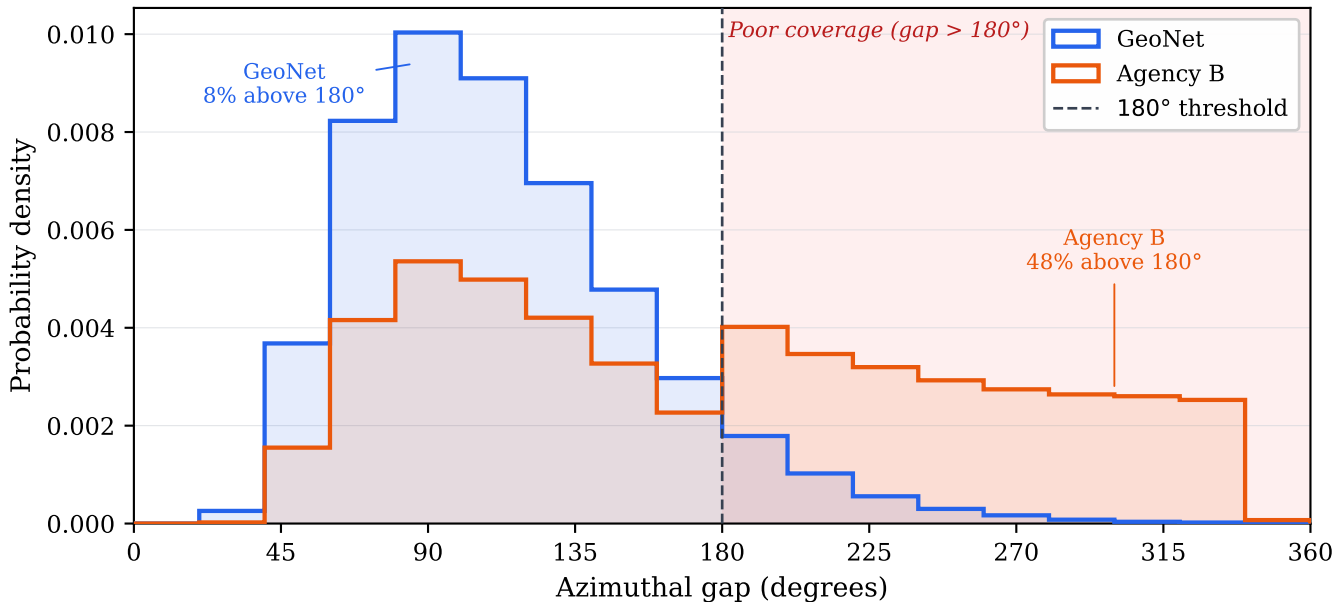
Azimuthal gap distribution: GeoNet vs Agency B
