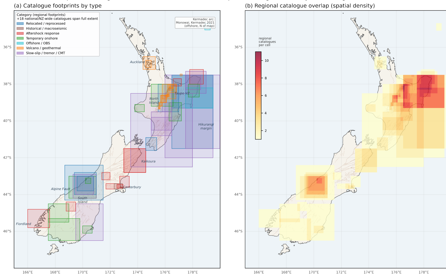
Figure 1: Spatial coverage of a companion inventory of New Zealand earthquake catalogues (81 catalogues, 1960–2026). (a) Footprint of each regional catalogue (a representative bounding box) over the coastline and active faults, coloured by type; 18 national or NZ-wide catalogues span the full extent and are not drawn, and two Kermadec-arc catalogues lie north of the map. (b) Number of regional catalogues overlapping each 0.1^\circ cell, highlighting intensively studied areas (Taupō Volcanic Zone, Hikurangi margin, Canterbury, central Alpine Fault) against thinly catalogued offshore tracts, Fiordland, and the far south. This many-catalogues-per-area pattern is the motivation for a merging-and-quality platform.
