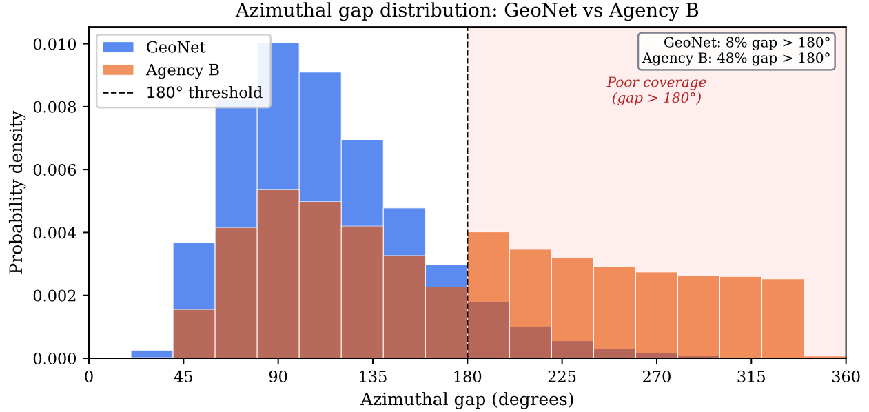
Figure 5: Distribution of azimuthal gap (in degrees) for the GeoNet catalogue (blue) and Agency B (orange) before merging. The long tail > 180^\circ in Agency B reflects limited offshore station coverage. Events with gap > 180^\circ receive a low network-geometry sub-score Q_{\text{net}} (Section 2.6) and are typically graded C or below. The shaded region marks the poor-coverage zone. Percentages shown are the fraction of events in each catalogue with gap exceeding 180^\circ .
