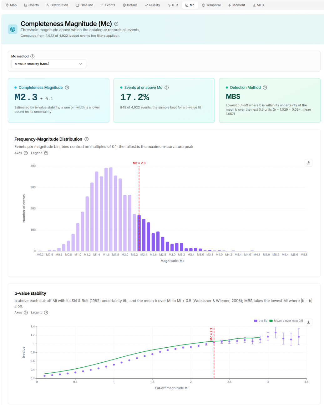
Figure S2: Magnitude-of-completeness panel for the same catalogue, with the default method, b -value stability (the main paper’s M_c section; Woessner and Wiemer, 2005); the goodness-of-fit test and maximum curvature, with a correction from 0 to 0.5, are the alternatives. M_c = M2.3 \pm 0.1 (one bin width, a lower bound on its uncertainty) is the lowest cut-off at which \hat{b} lies within its Shi and Bolt (1982) uncertainty of its mean over the cut-offs M2.3 – M2.8 : the method card quotes \hat{b} = 1.029 , \delta b = 0.034 and a mean of 1.057. At or above M_c lie 17.2% of the events (845 of 4,922), the sample a b -value fit keeps; the share is not a completeness score. The distribution is drawn in bins centred on multiples of 0.1, and the fullest bin of the non-cumulative distribution is M1.7 , so maximum curvature with its default +0.2 correction would give M1.9 , and the goodness-of-fit test gives M2.2 at the 95% level. Below the distribution (bottom of the figure) the tab plots the stability test itself, \hat{b} \pm \delta b and the mean over the next 0.5 units at every cut-off with at least 50 events above it, whichever method set M_c ; M_c is the first cut-off whose error bar reaches the mean. b -value stability is conservative on large samples, because \delta b falls as 1/\sqrt{N} : on the full-scale GeoNet-like catalogue of the main paper, 23 times larger, it gives M2.7 . The estimate is shown with its method and the values behind it, so that the completeness assumption behind any subsequent b -value is visible at the point of use.
