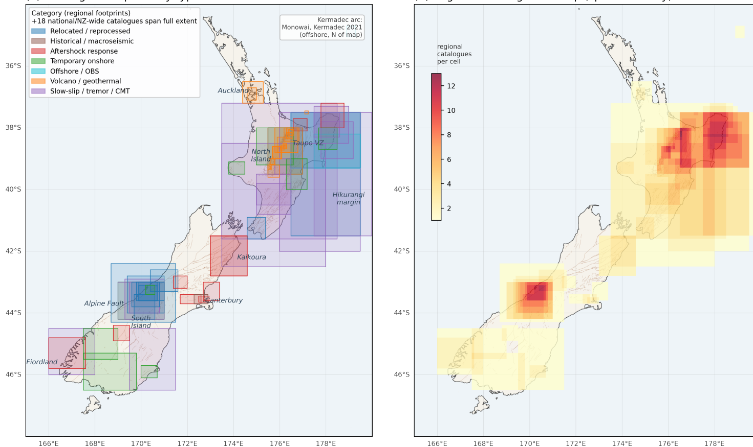
Spatial coverage of the Aotearoa New Zealand earthquake-catalogue inventory (93 catalogues, 1960-2026)
