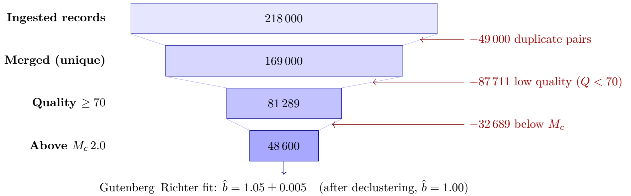
Figure 8: Quantitative event-count flow through the CofC pipeline for the synthetic worked example (Section 7). Bar widths are proportional to the number of events; each stage removes a characterised subset (red) before the Gutenberg–Richter b -value is estimated on the surviving population. All counts are properties of the controlled synthetic inputs, not real New Zealand seismicity.
