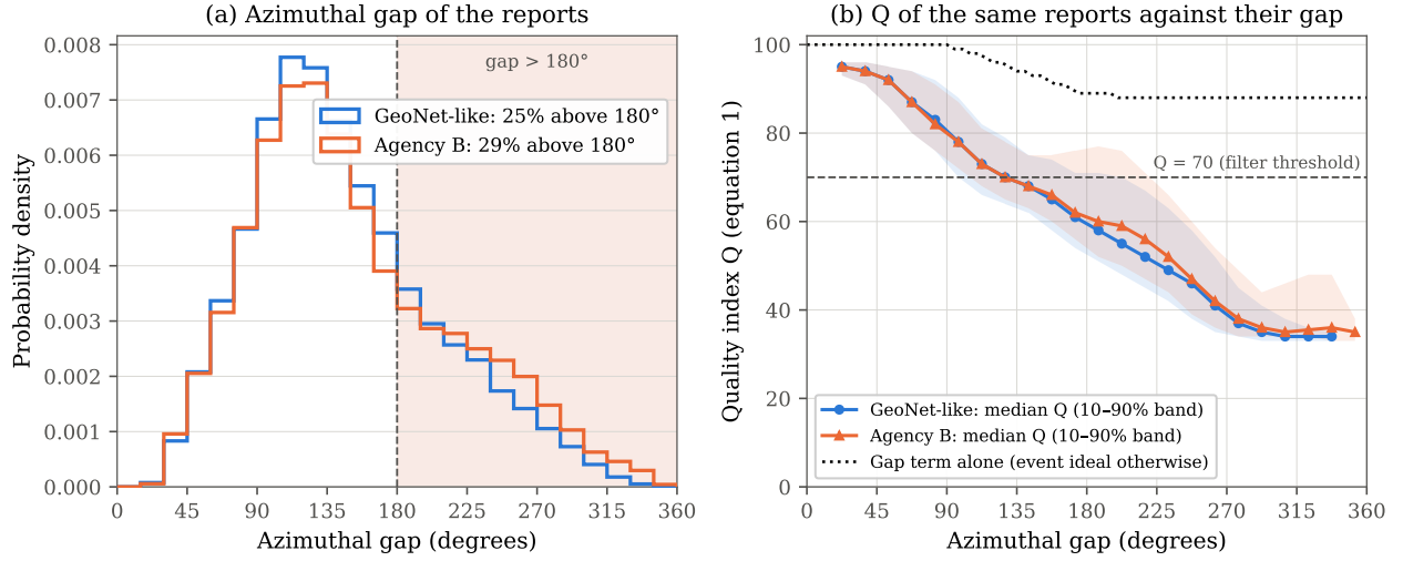
Figure 5: Azimuthal gap and the quality index on the synthetic example (Section 7). (a) Distribution of azimuthal gap for the GeoNet-like (blue) and Agency B (orange) entries before merging; the gaps are computed from each synthetic network’s geometry, so events offshore or outside a network have large gaps, and the shaded region marks gaps above 180°. (b) The quality index Q (equation (1)) that the platform assigns the same entries on import, against their gap: median and 10–90% range in 15° bins. The dotted line is the Q of an event that is ideal in every other respect: the gap term alone can lower Q by at most 12.5 points (to 88), so most of the fall comes from the larger location uncertainties and smaller station counts that the high-gap entries carry. The dashed line is the Q \geq 70 threshold applied in the example.
