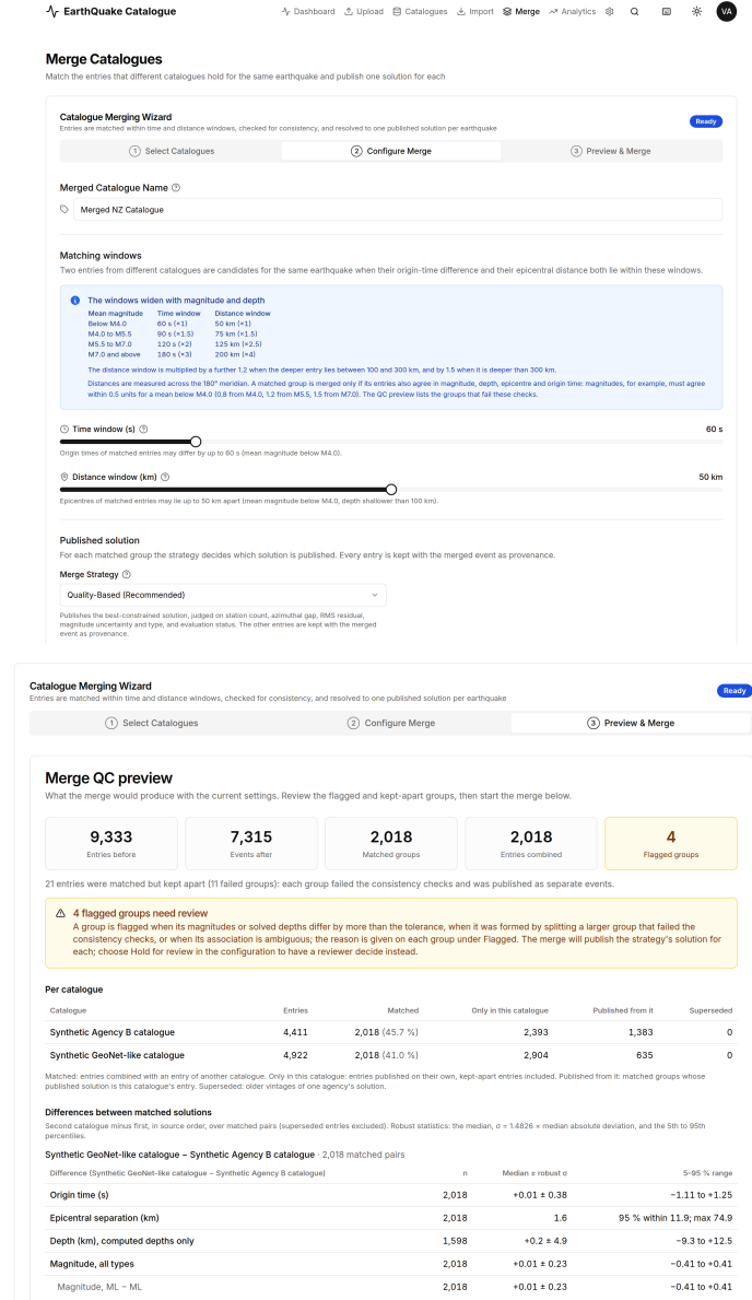
Figure 3: The merge workflow in the browser (the release described here). Top : the Configure step, with the matching windows (equations (2)–(3); here 60 s and 50 km), a table of the windows the adaptive multipliers give in each magnitude band (with the further widening for depth), and the strategy that selects the published solution (Table 4; here Quality-based). Bottom : the Preview step, a dry run of the merge with its QC summary, before anything is written. The totals read Entries before 9 333, Events after 7 315, Matched groups 2 018, Entries combined 2 018 and Flagged groups 4, and 21 entries of 11 groups that failed the gates are kept apart, published as separate events. The summary goes on to each catalogue’s matched entries (41.0% of the GeoNet-like and 45.7% of the Agency B entries) and the differences between matched solutions, and the groups to review follow under Flagged (4), Kept apart (11) and Matched (2 014), largest disagreement first. Data are a reduced-scale version of the synthetic pair of the worked example (Section 7), 4 922 GeoNet-like and 4 411 Agency B events built by the same generator with each true earthquake kept with probability 1/23.
