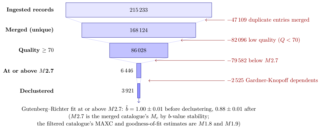
Figure 8: Event-count flow through the CofC pipeline for the synthetic worked example (Section 7), every count computed by the platform. Bar widths are proportional to the number of events; each stage removes the subset shown in red. The cut-off M2.7 is the platform’s b -value-stability estimate of M_c for the merged catalogue, the magnitude from which its b -value is stable (Figure 7c), well above the MAXC and goodness-of-fit estimates. All counts are properties of the controlled synthetic inputs, not real New Zealand seismicity.
