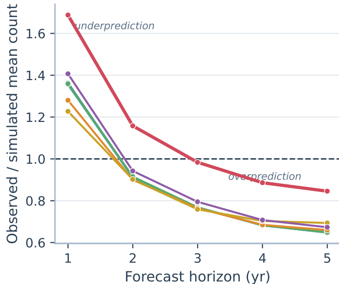
(a) Count-ratio evolution
