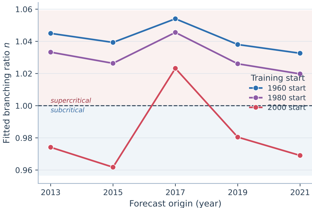
Branching ratio vs training window, across origins
