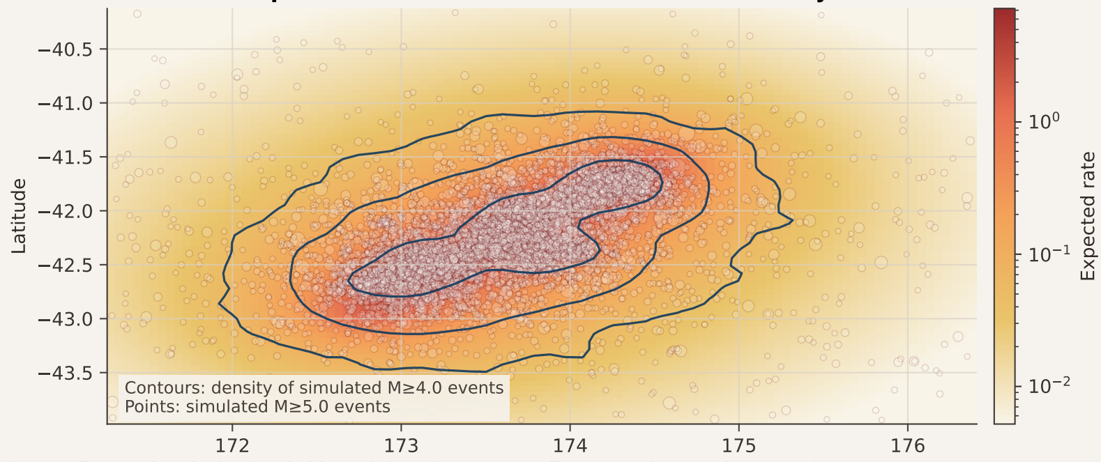
Spatial Rate Field and Realized Event Density
