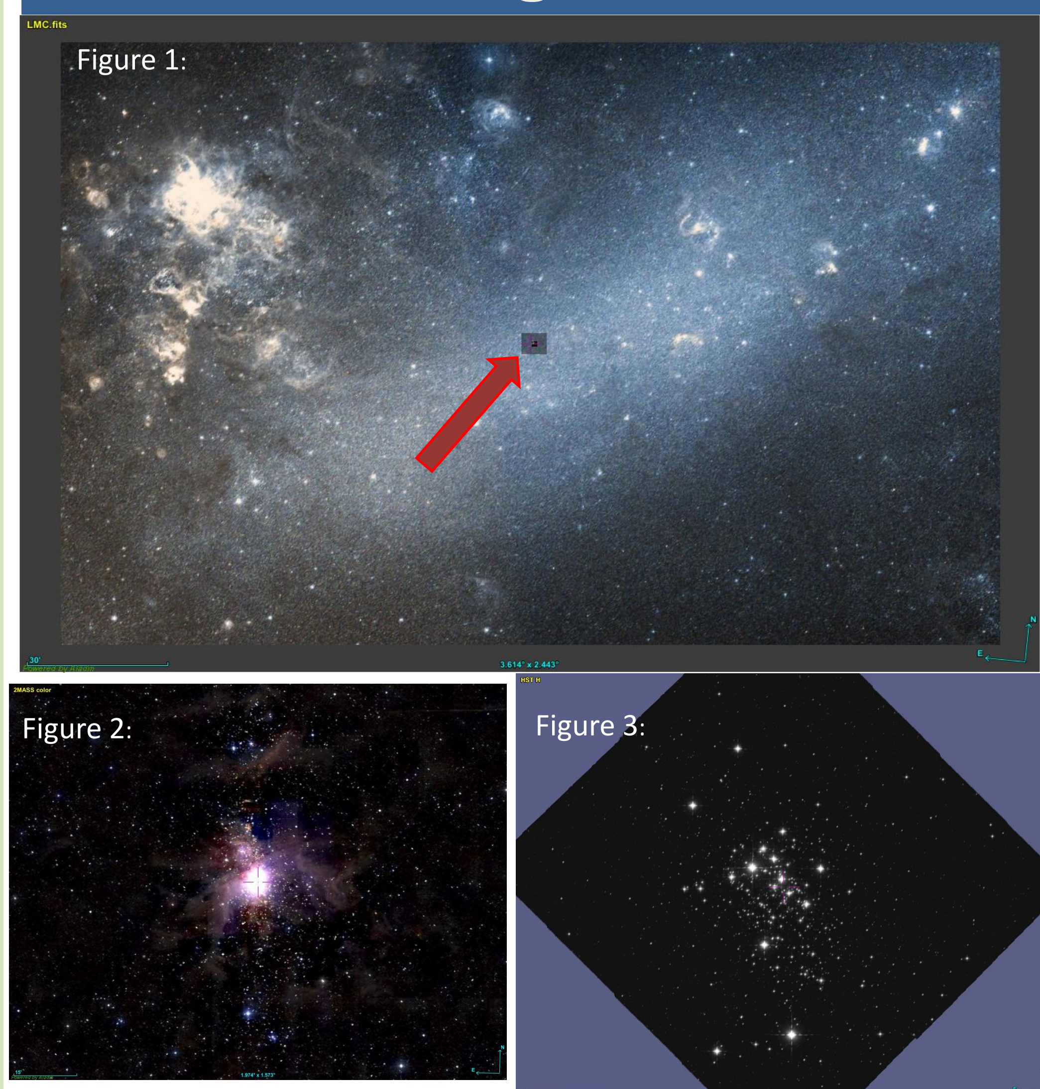
Figure 1 (top). 30 Doradus (top left), the most active LMC star-forming region; Wd1 and the ONC, projected to the LMC distance are shown by a red arrow (DSS2 color). Figure 2 (bottom left): Orion Nebula (2MASS IR); Figure 3 (bottom right): Westerlund 1 (Hubble Space Telescope, F160W)
