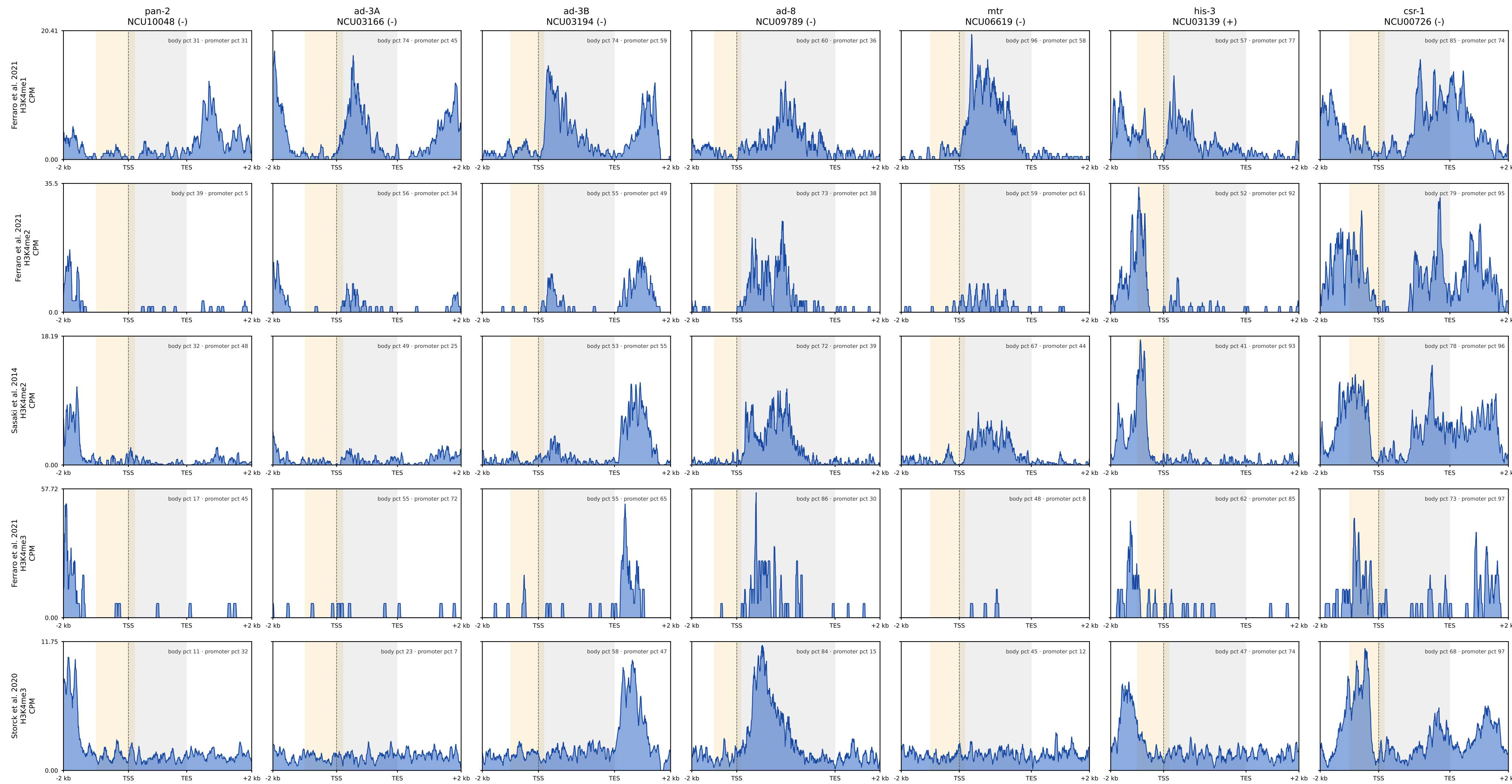
Each row has one shared y-axis across all seven loci; y-axes are not shared between runs. Gold: promoter (-1 kb to +200 bp); gray: annotated gene body. Annotations are within-run genome-wide midrank percentiles.
