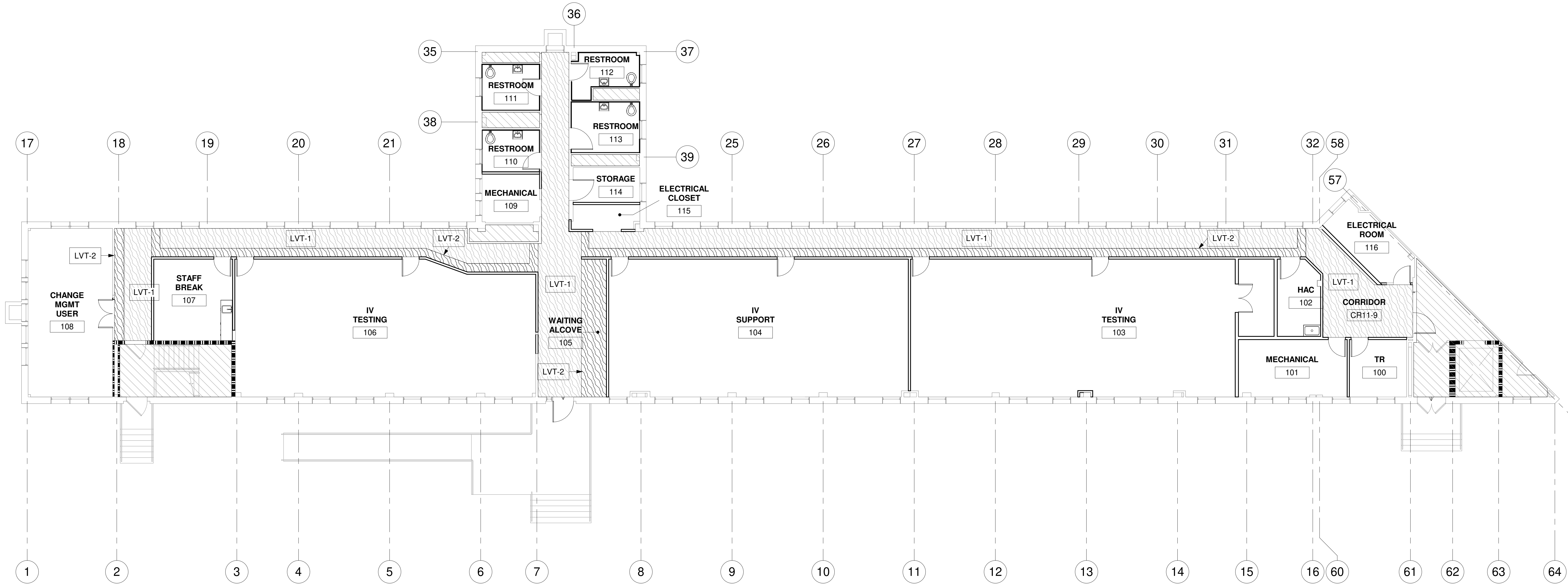
1 FLOOR PLAN - PHASE I - FINISH PLAN 1/8" = 1'-0"
