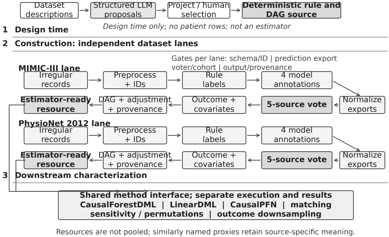
Figure 1: CliniCause resource construction. Dataset-specific preprocessing and deterministic proxy rules transform irregular ICU records; four time-series models add normalized predictive annotations, and per-dataset deterministic five-source aggregation packages the aligned proxy layer with outcomes, observed covariates, and inspectable DAG metadata. The design-time LLM proposes candidates only; deterministic selected source governs runtime. Validation gates protect schema, cohort, prediction-export, aggregation, and provenance handoffs before separate dataset-specific estimator-ready resources are used for observational analysis.
