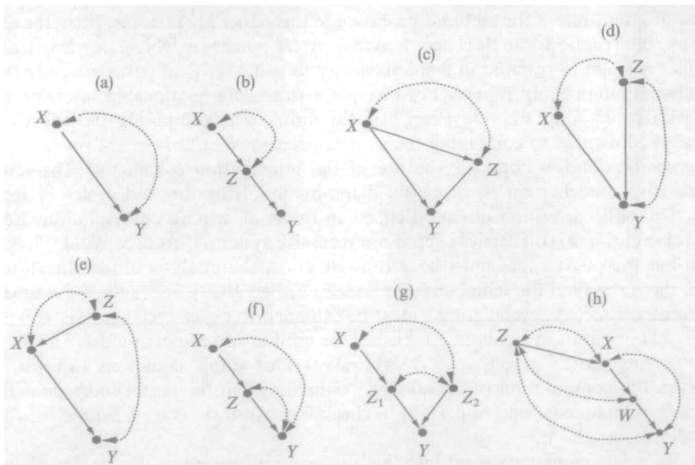
Fig. 7. Typical models in which \text{pr}(y|\tilde{x}) is not identifiable.
