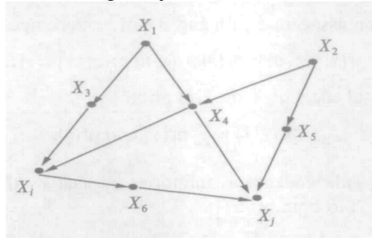
Fig. 2. A diagram representing the back-door criterion; adjusting for variables \{X_3, X_4\} or \{X_4, X_5\} yields a consistent estimate of \text{pr}(x_j|x_i) .
