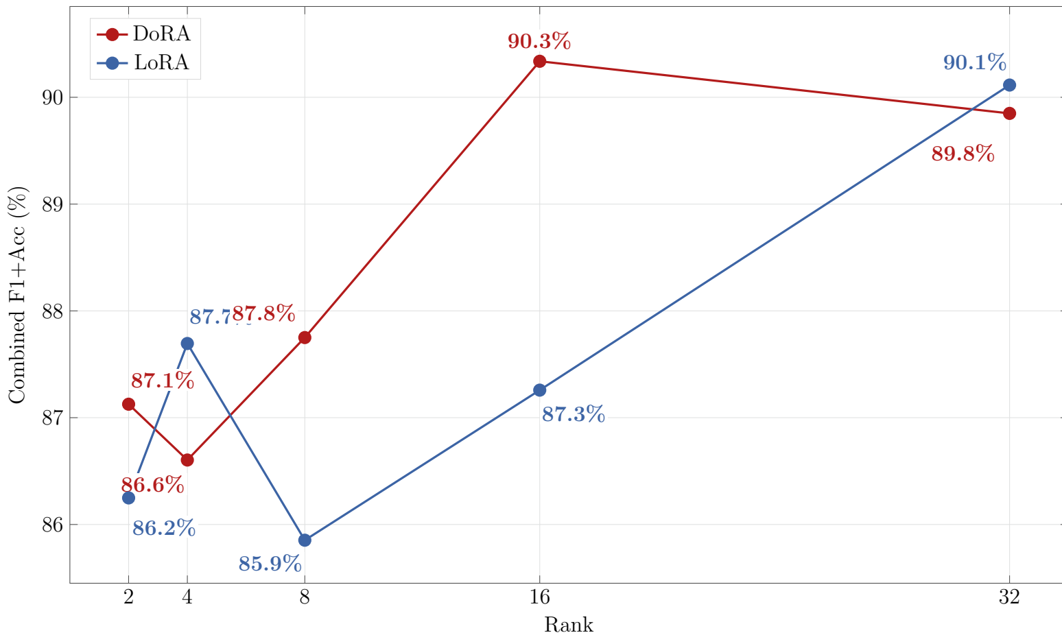
MRPC Combined Score vs Rank (RoBERTa-base, \alpha = 2 \times \text{rank} )
