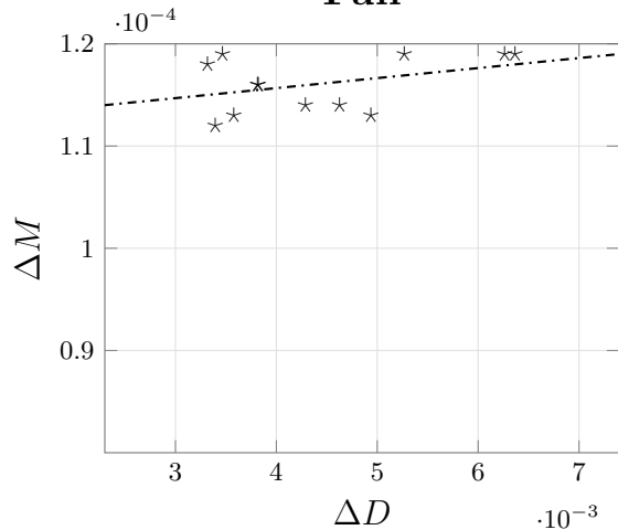
Full
