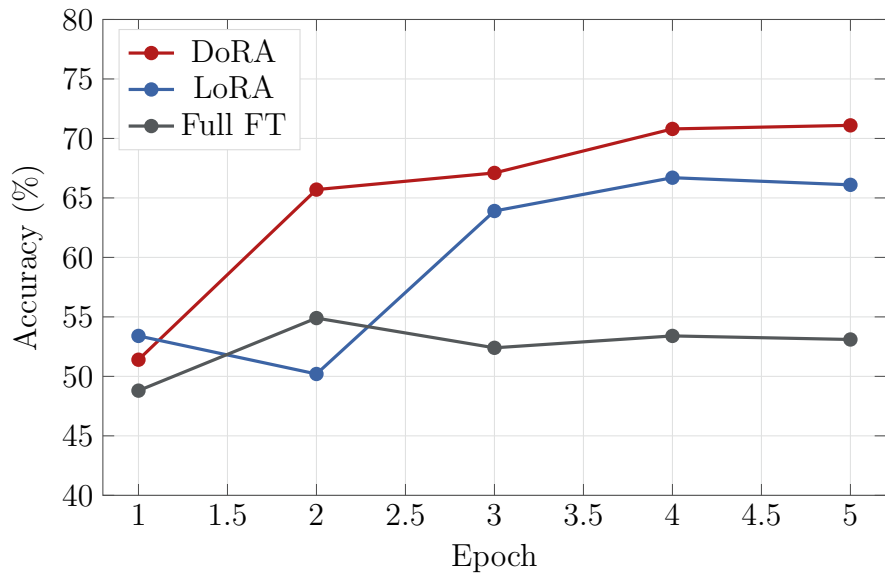
RTE Eval Accuracy over Epochs
