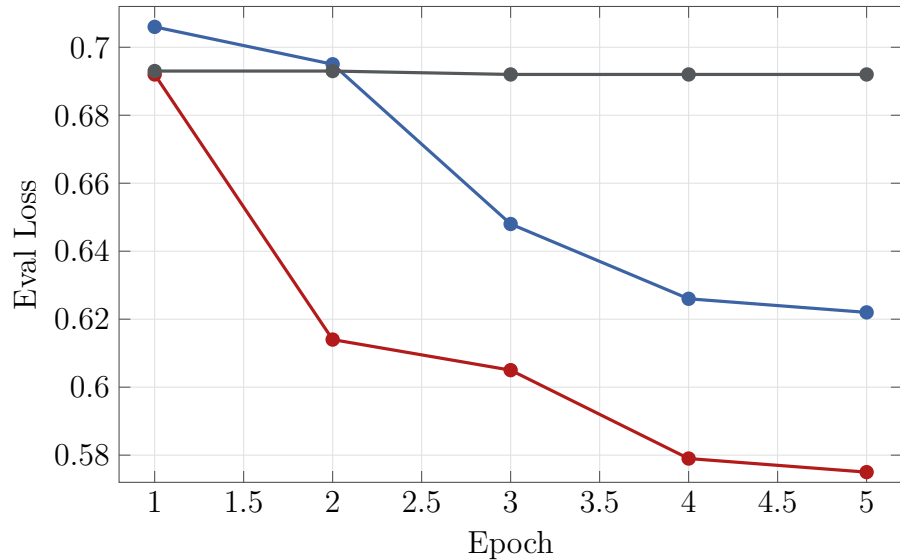
RTE Eval Loss over Epochs
