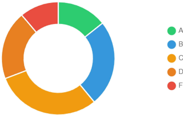
Grade Distribution
