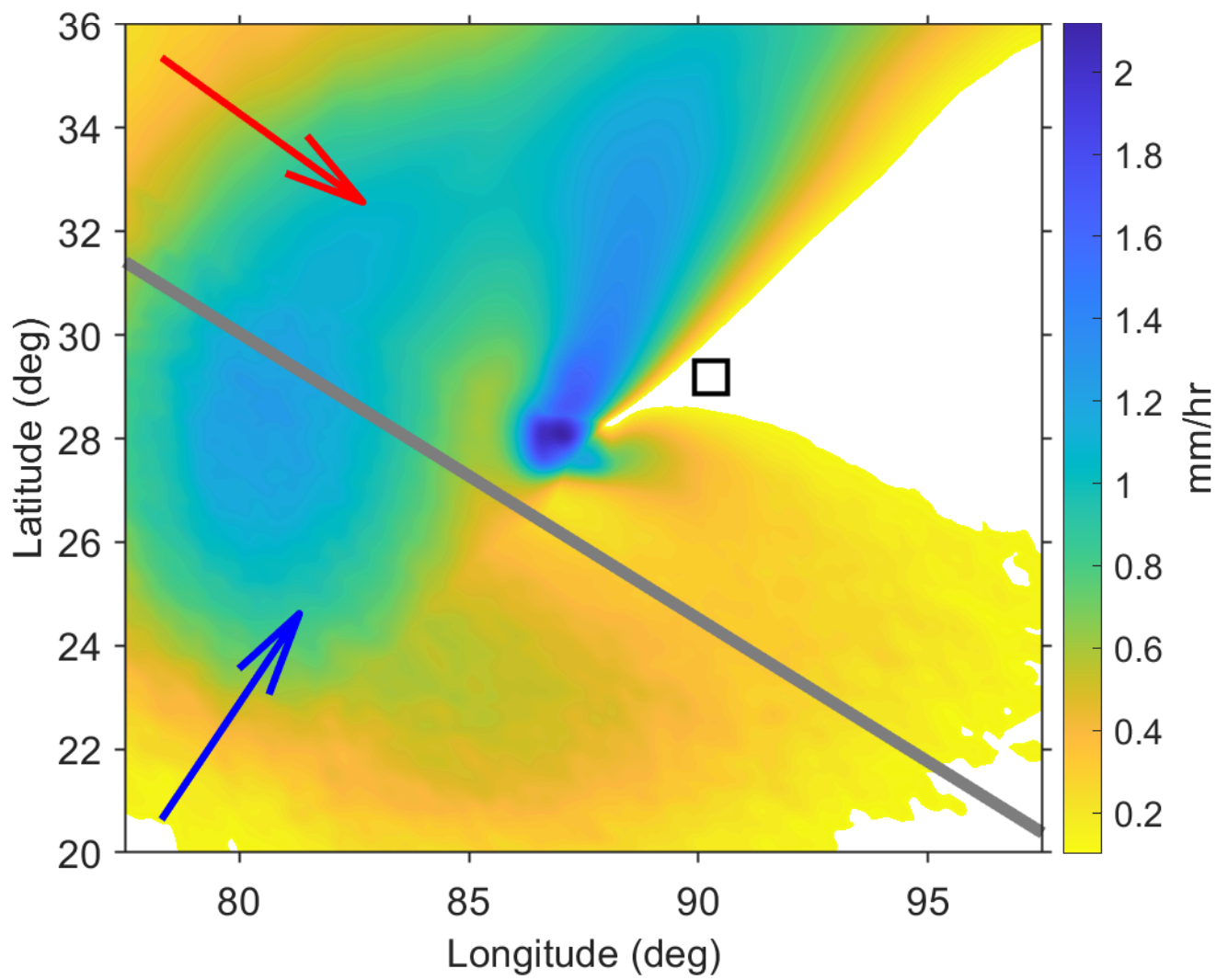
Fig. 2. Precipitation rate
