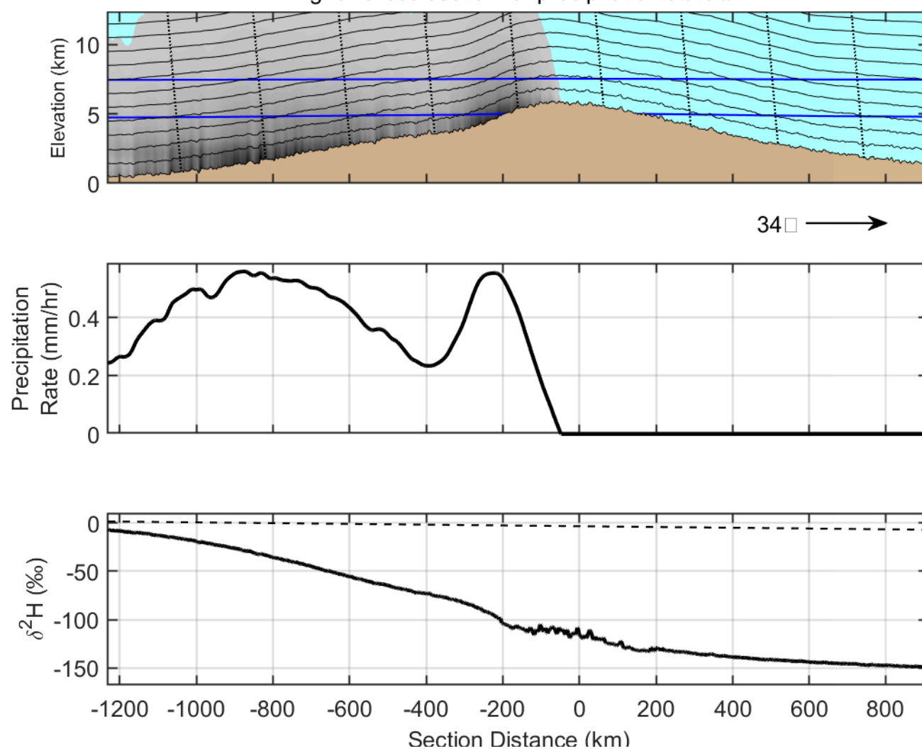
Fig. 5. Cross section for precipitation state #1
