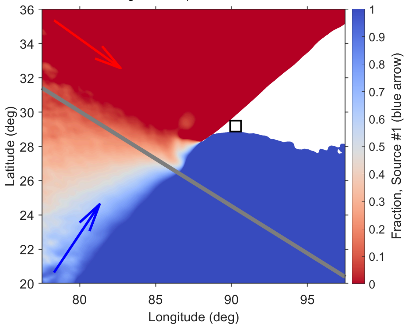
Fig. 9. Precipitation source
