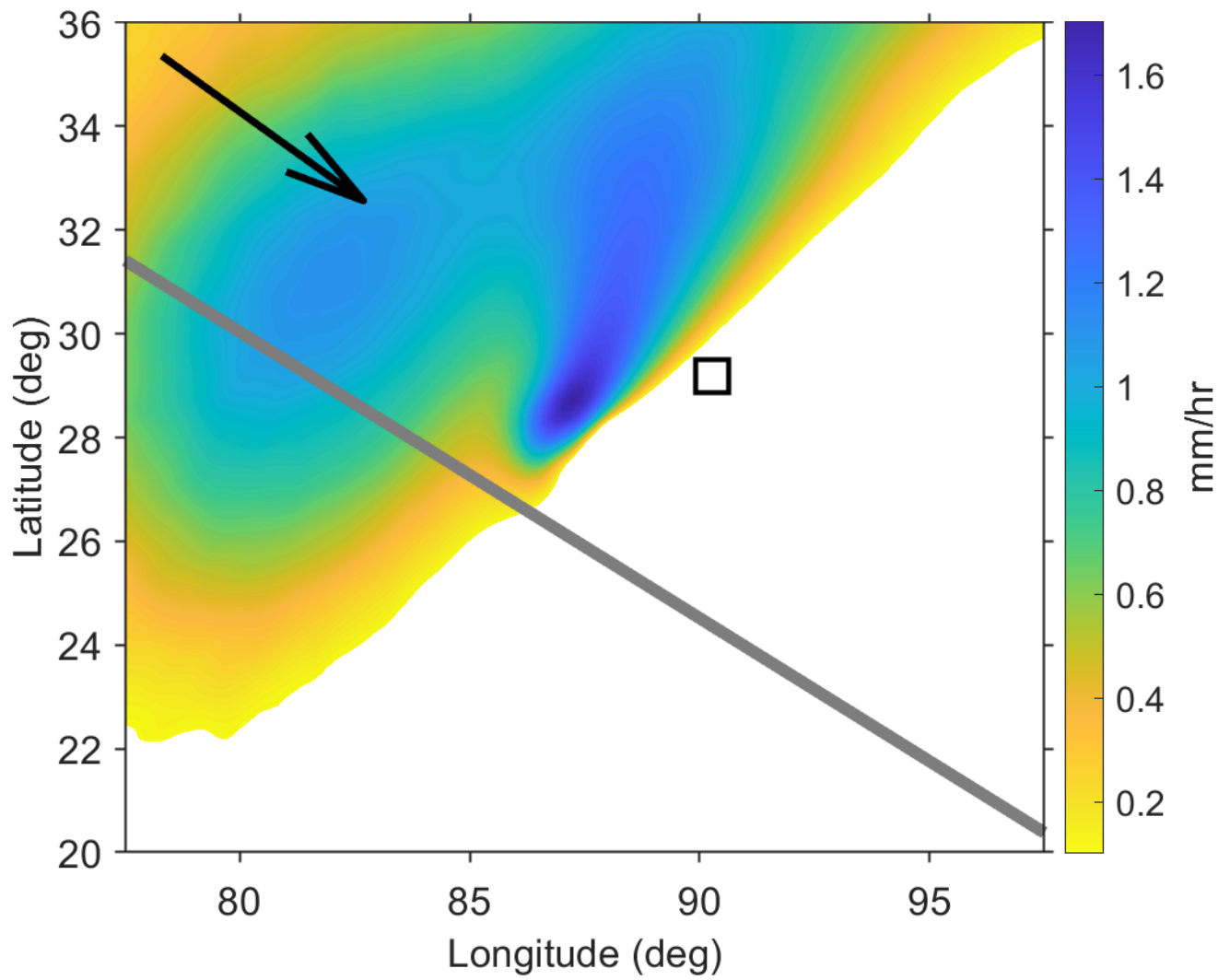
Fig. 11. Precipitation rate, state #2
