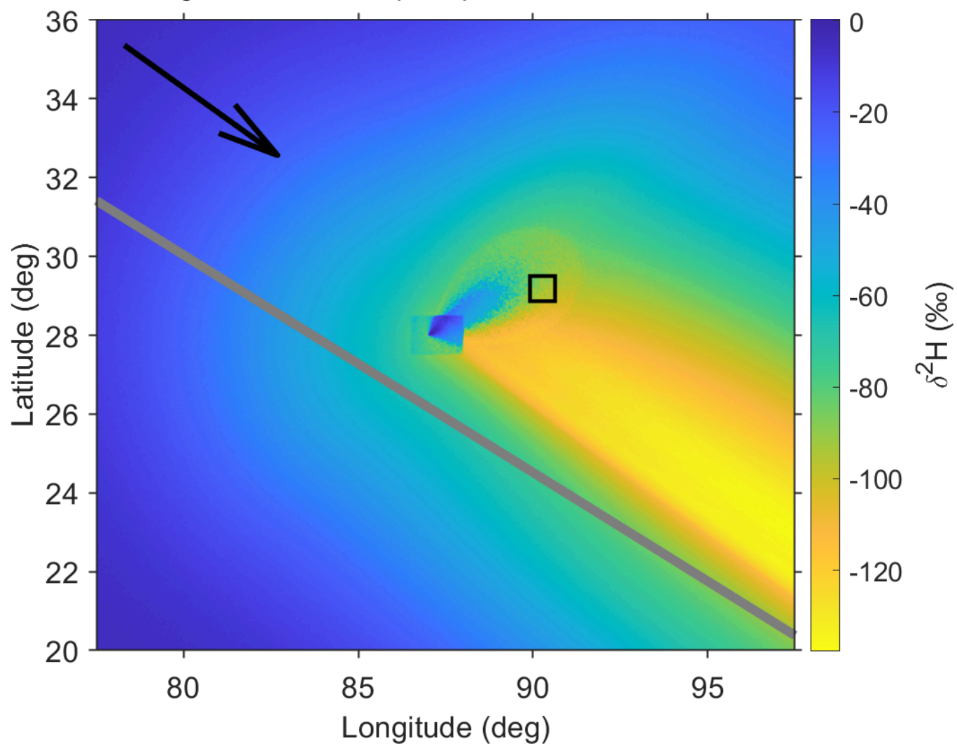
Fig. 15. Predicted precipitation \delta^2\text{H} , state #2
