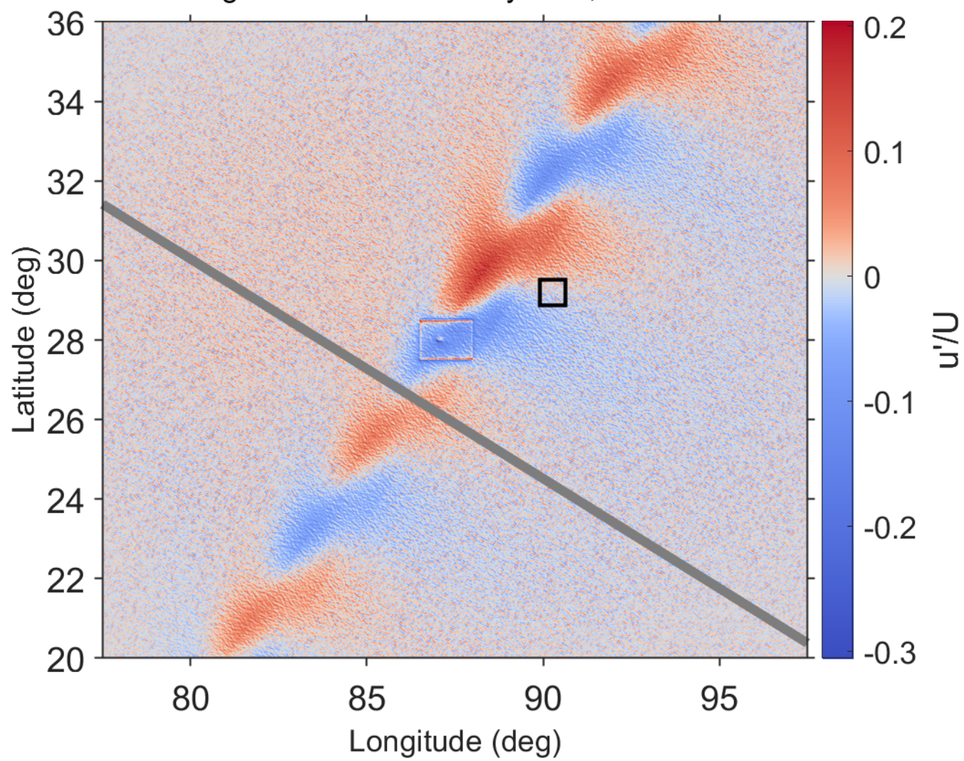
Fig. 18. Surface velocity ratio, state #1
