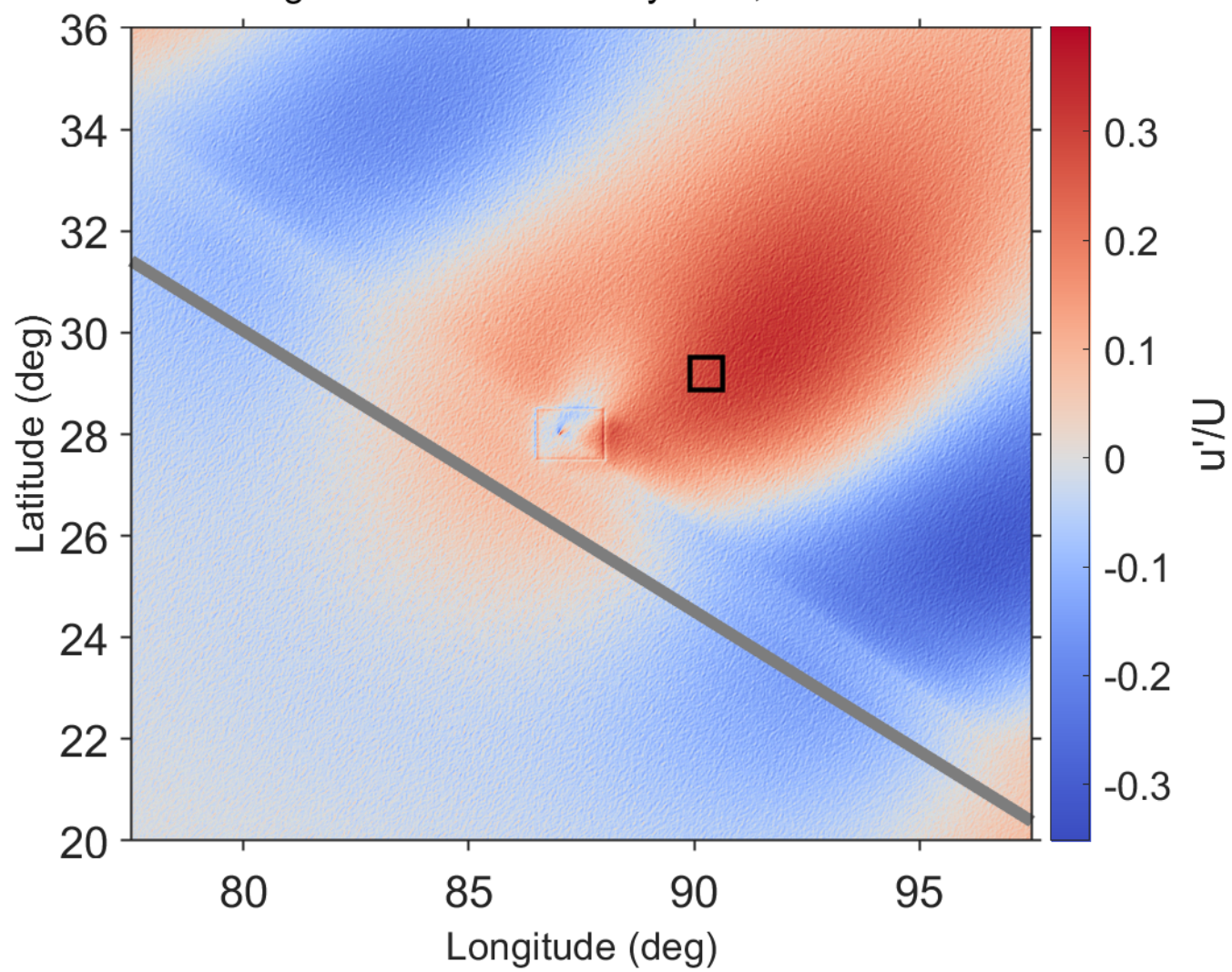
Fig. 19. Surface velocity ratio, state #2
