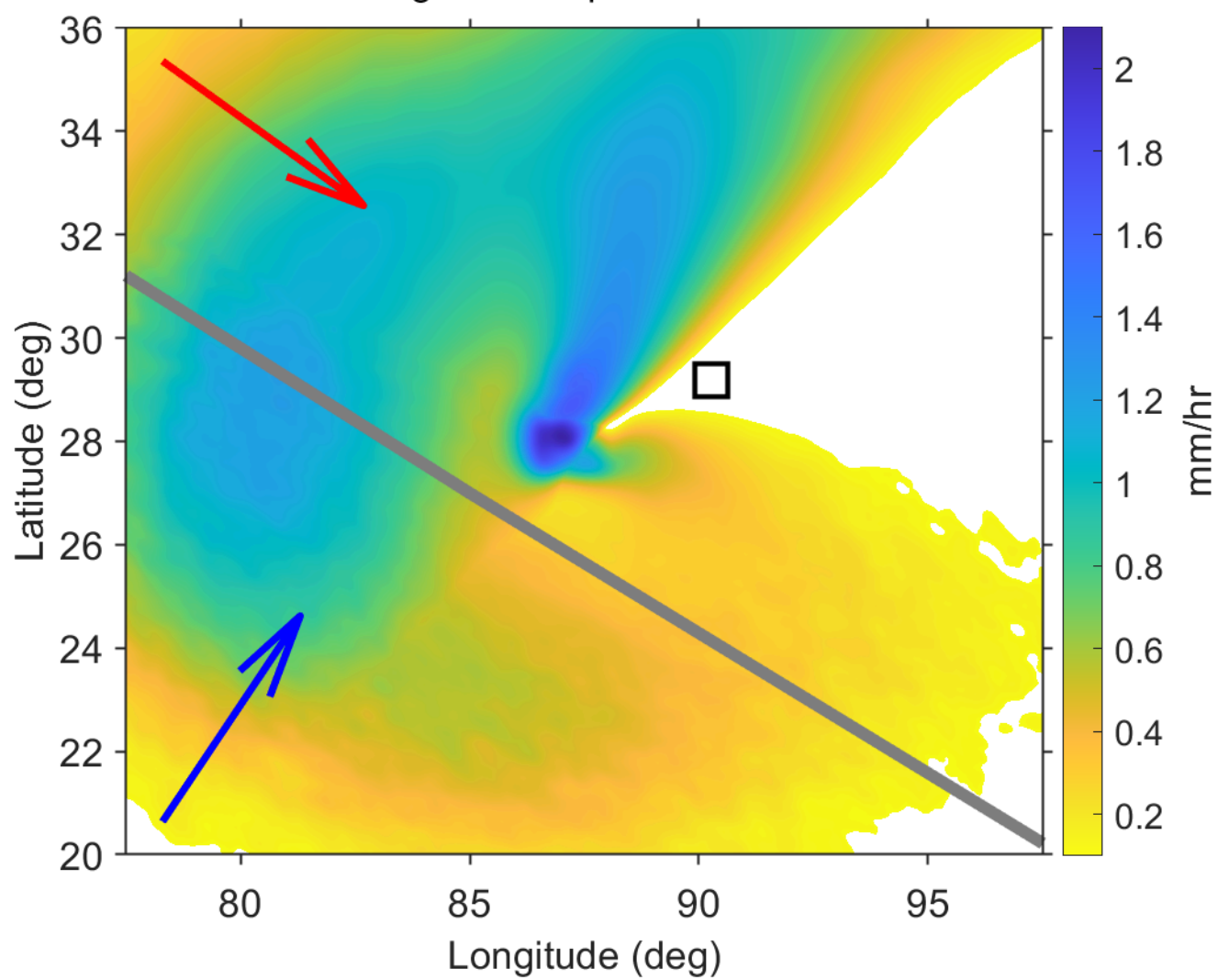
Fig. 2. Precipitation rate
