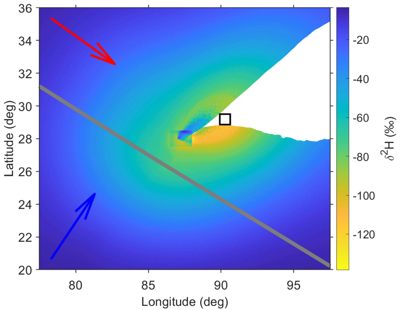
Fig. 7. Predicted precipitation \delta^2\text{H}
