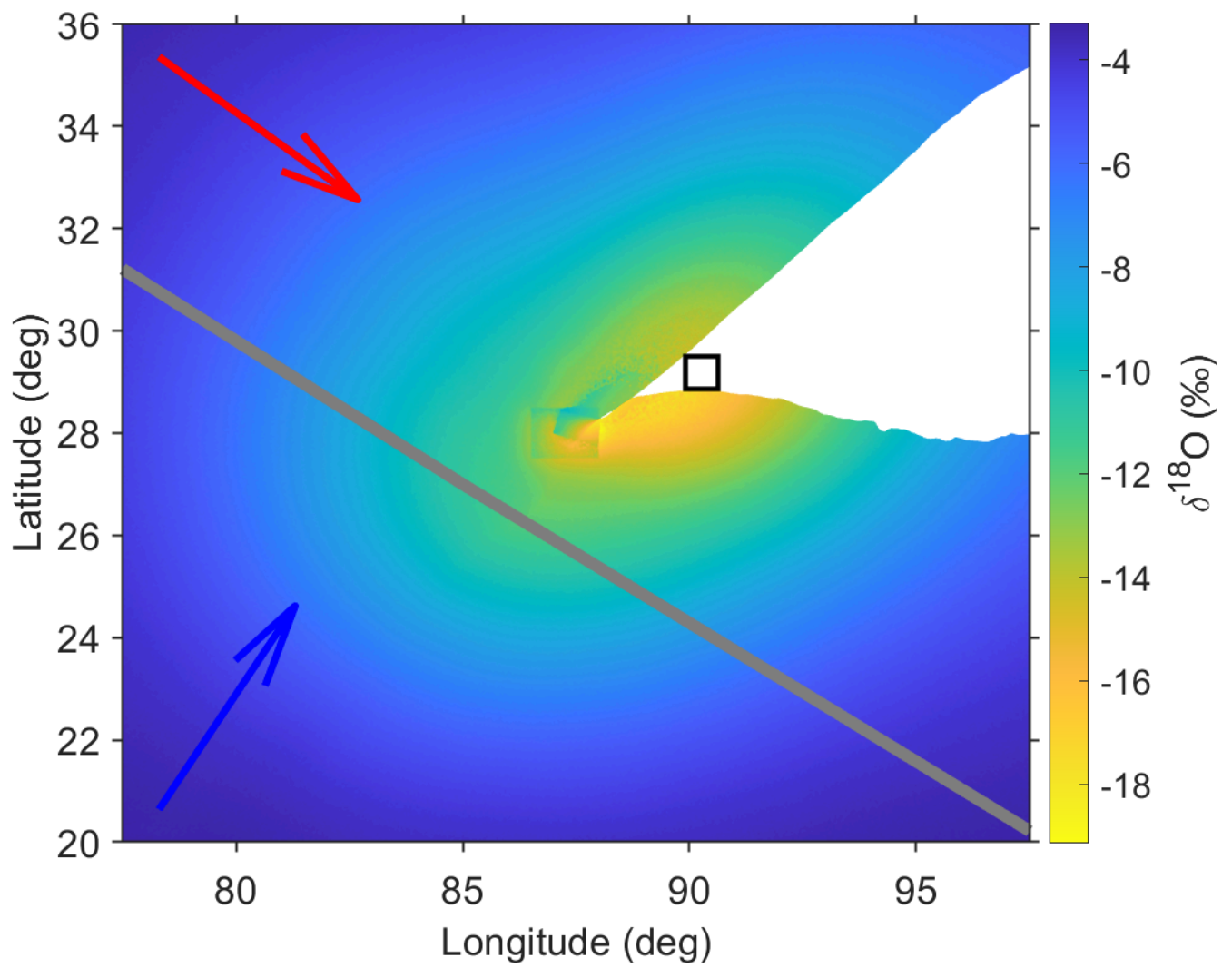
Fig. 8. Predicted precipitation \delta^{18}\text{O}
