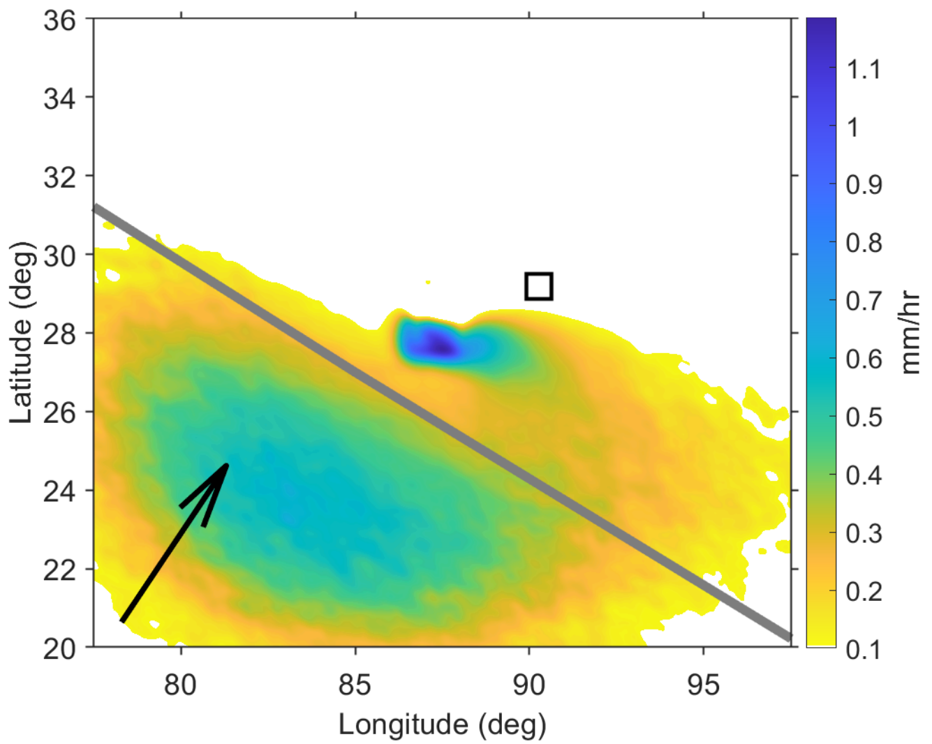
Fig. 10. Precipitation rate, state #1
