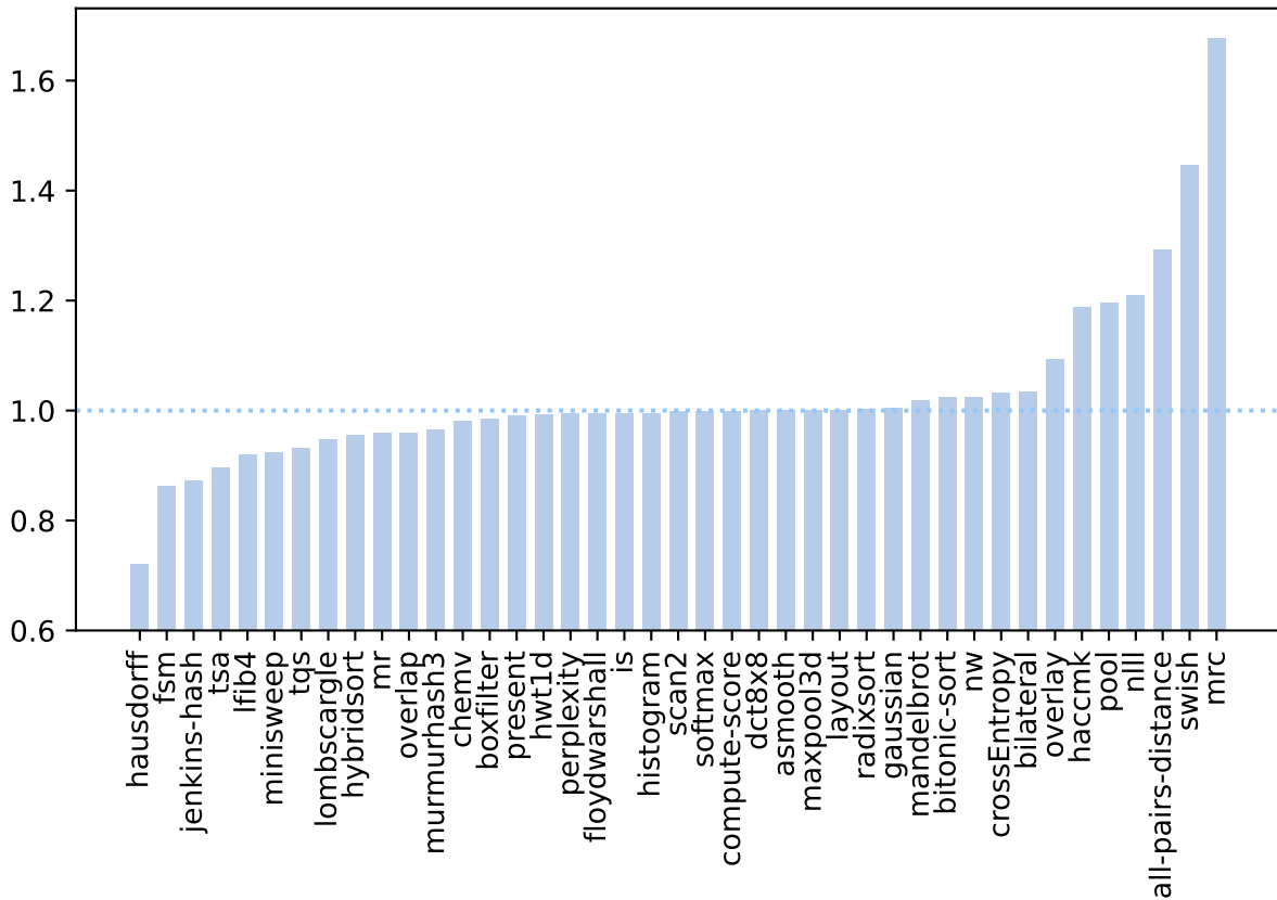
HeCBench, i9 12900 iGPU, chipStar vs SYCL speedup
