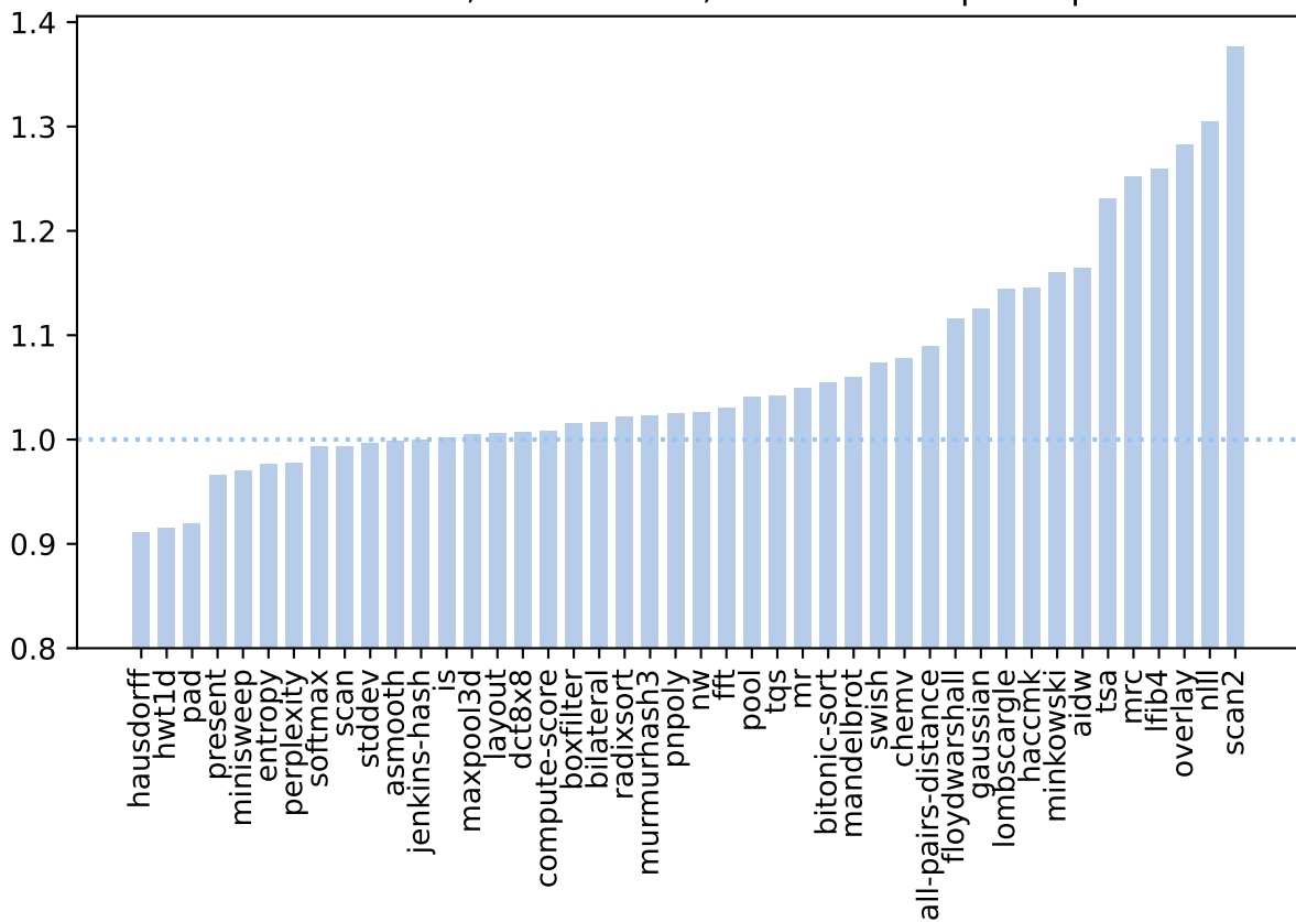
HeCBench, Intel Arc750, HIP vs SYCL speedup
