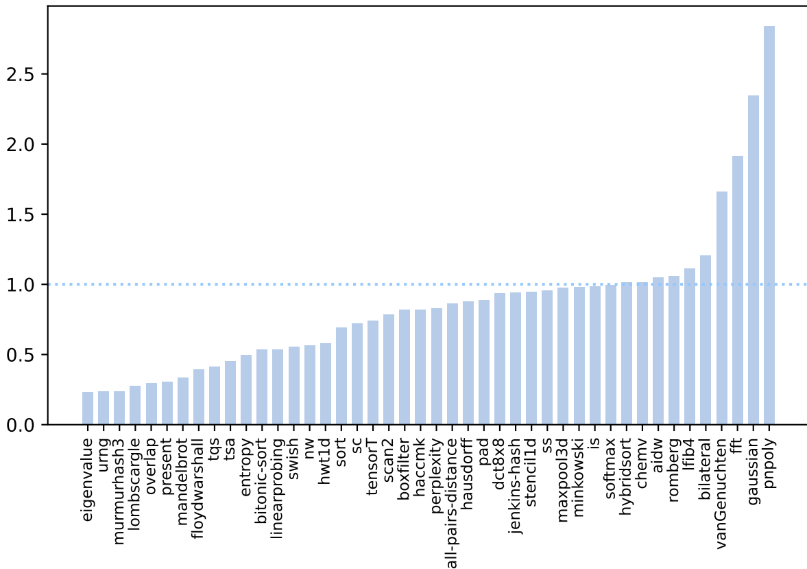
HeCBench, Radeon PRO VII, ROCm vs. chipStar/rusticl/radeonsi
