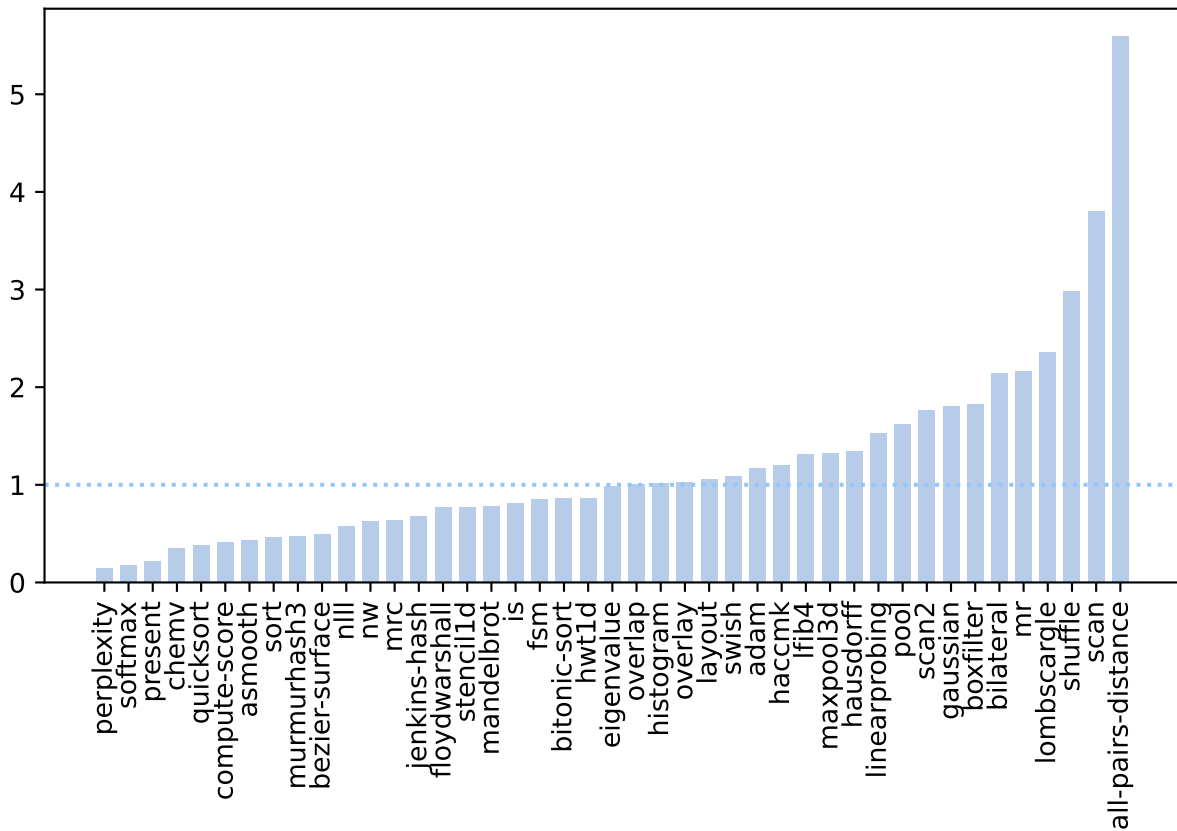
HeCBench, i9 12900, iGPU vs CPU speedup
