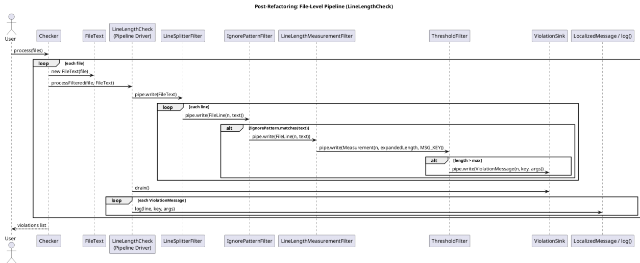
Figure: Post-refactor file-level check sequence — the driver routes the FileText into a LineSplitterFilter and the same threshold/sink tail used by the AST checks.
