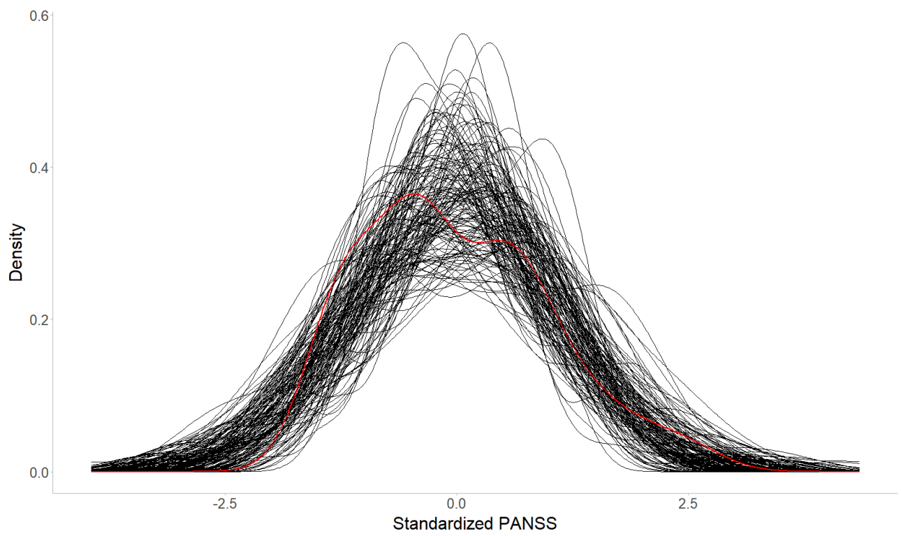
S_Figure 2: Posterior predictive check of PANSS. The red line shows the observed values.
