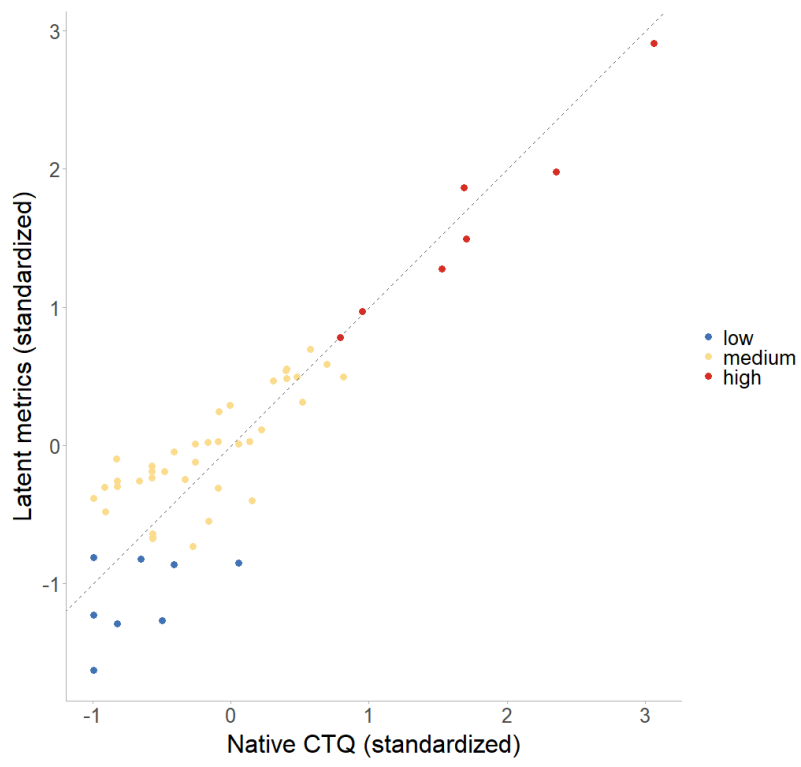
S_Figure 10: Native CTQ vs. posterior-mean latent metrics.
