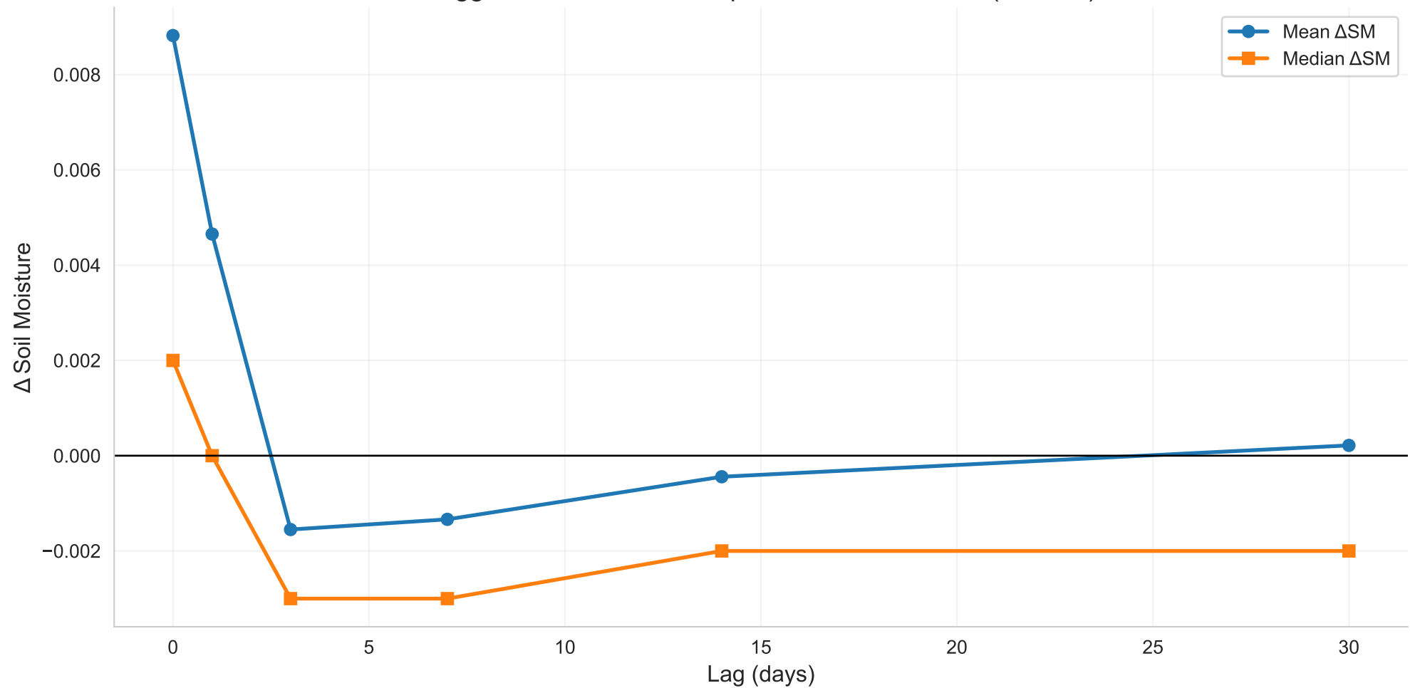
Lagged Soil Moisture Response to Rain Events ( \geq 4 mm)
