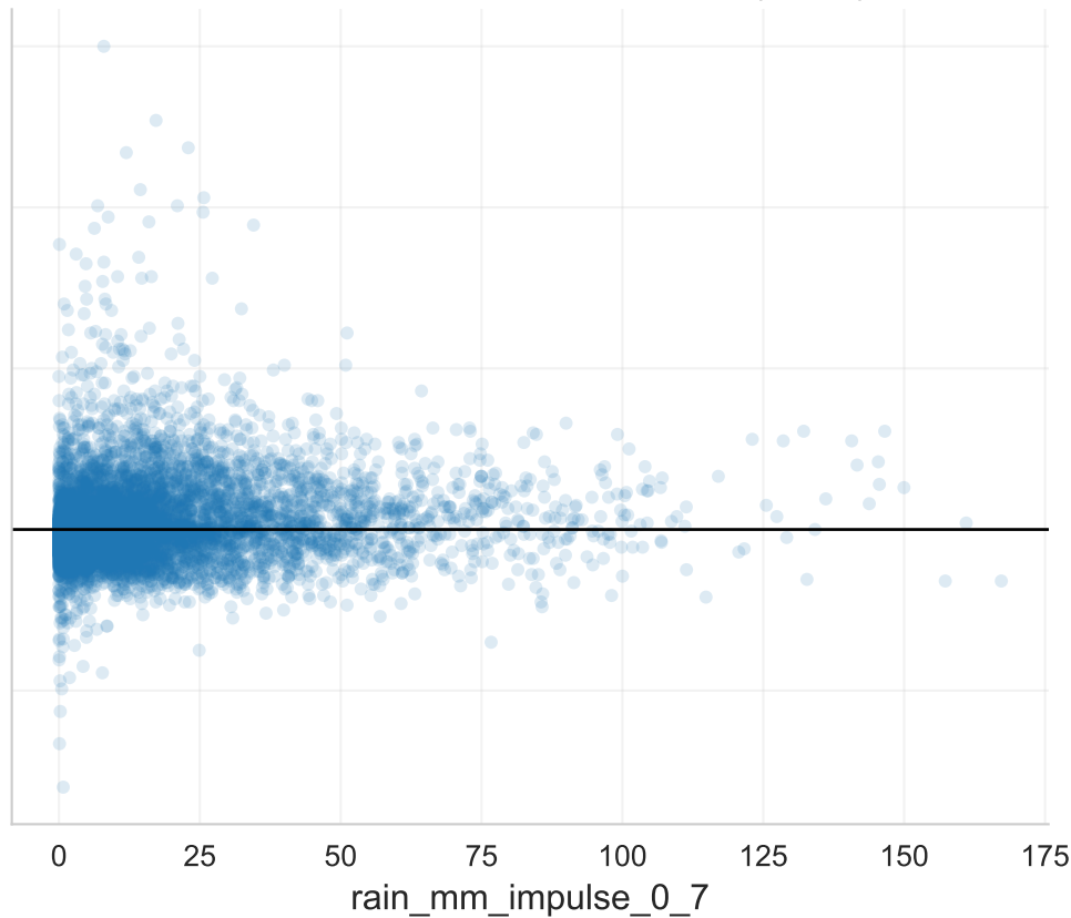
\Delta SM vs Rain Amount Impulse (0–7d)
