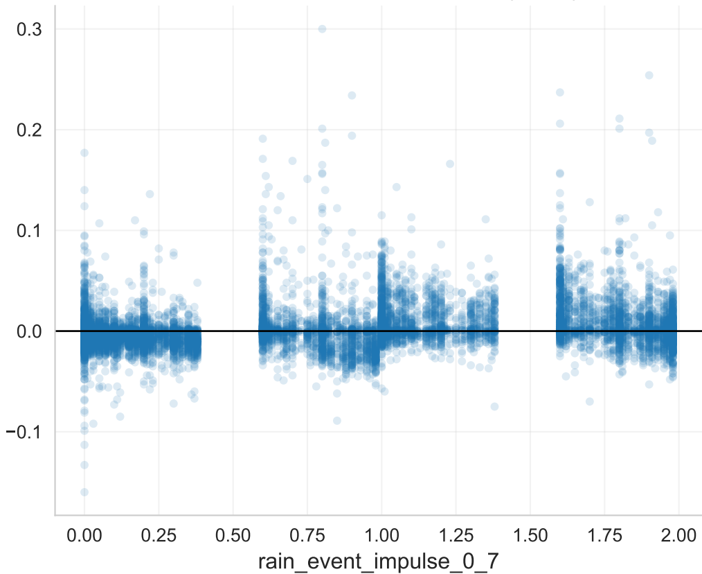
\Delta SM vs Rain Event Impulse (0–7d)
