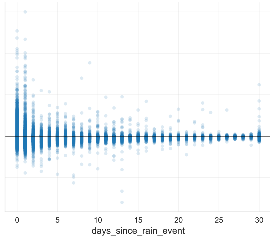
\Delta SM vs Days Since Rain Event
