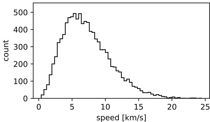
W0=10, rc=0.0005 kpc
