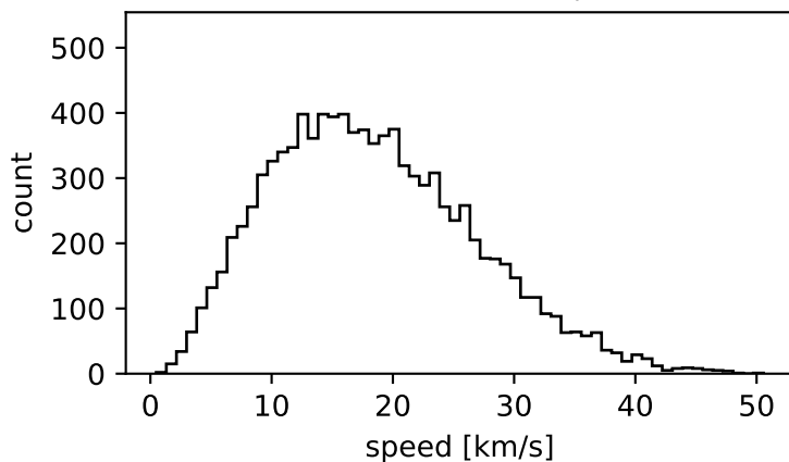
W0=10, rc=0.0005 kpc
