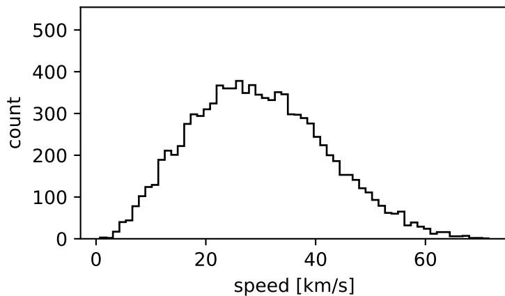
W0=7, rc=0.0005 kpc
