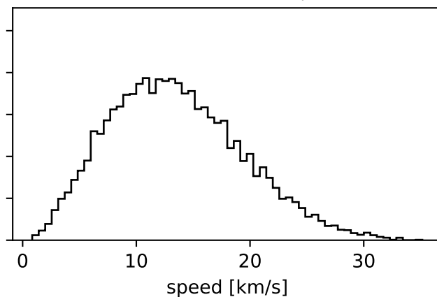
W0=10, rc=0.0010 kpc
