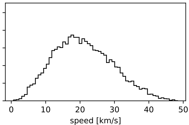
W0=7, rc=0.0010 kpc
