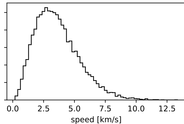
W0=10, rc=0.0020 kpc
