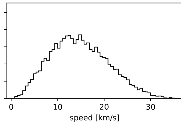
W0=7, rc=0.0020 kpc
