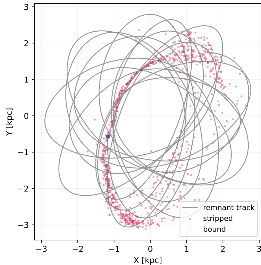
Galactocentric X-Y
