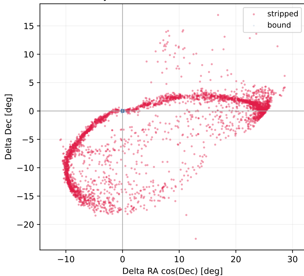
Sky offsets from remnant center
