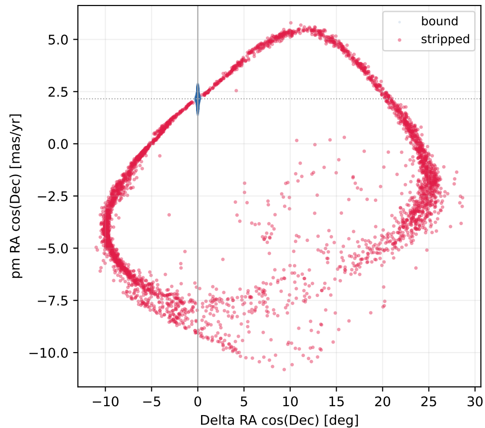
Position plus proper motion separates remnant and tail particles
