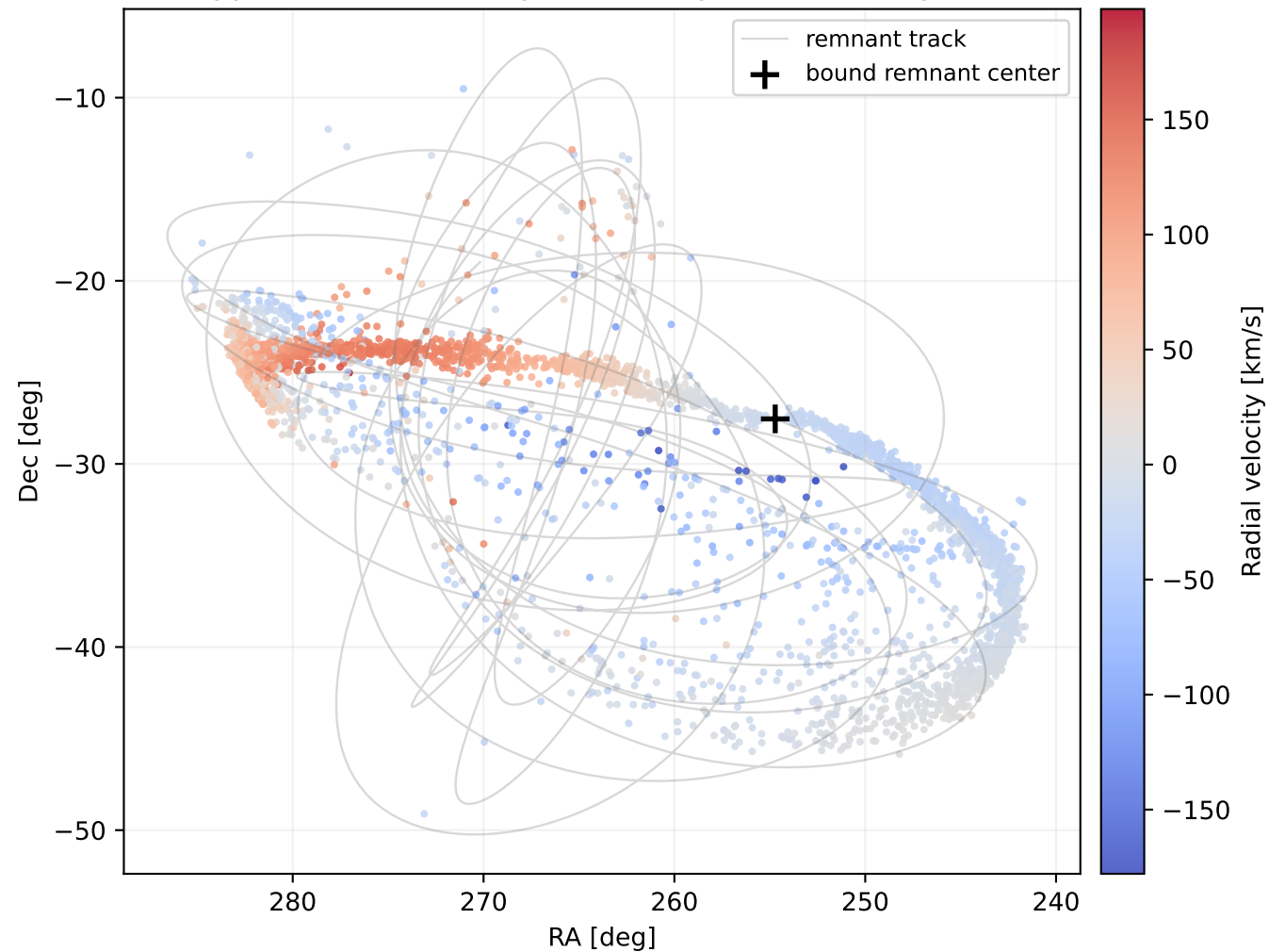
Stripped stars on the sky, colored by radial velocity [km/s]
