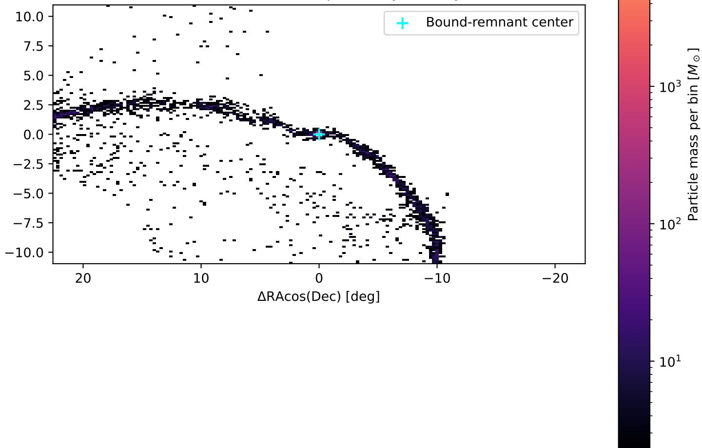
NGC 6569 final-snapshot sky density
