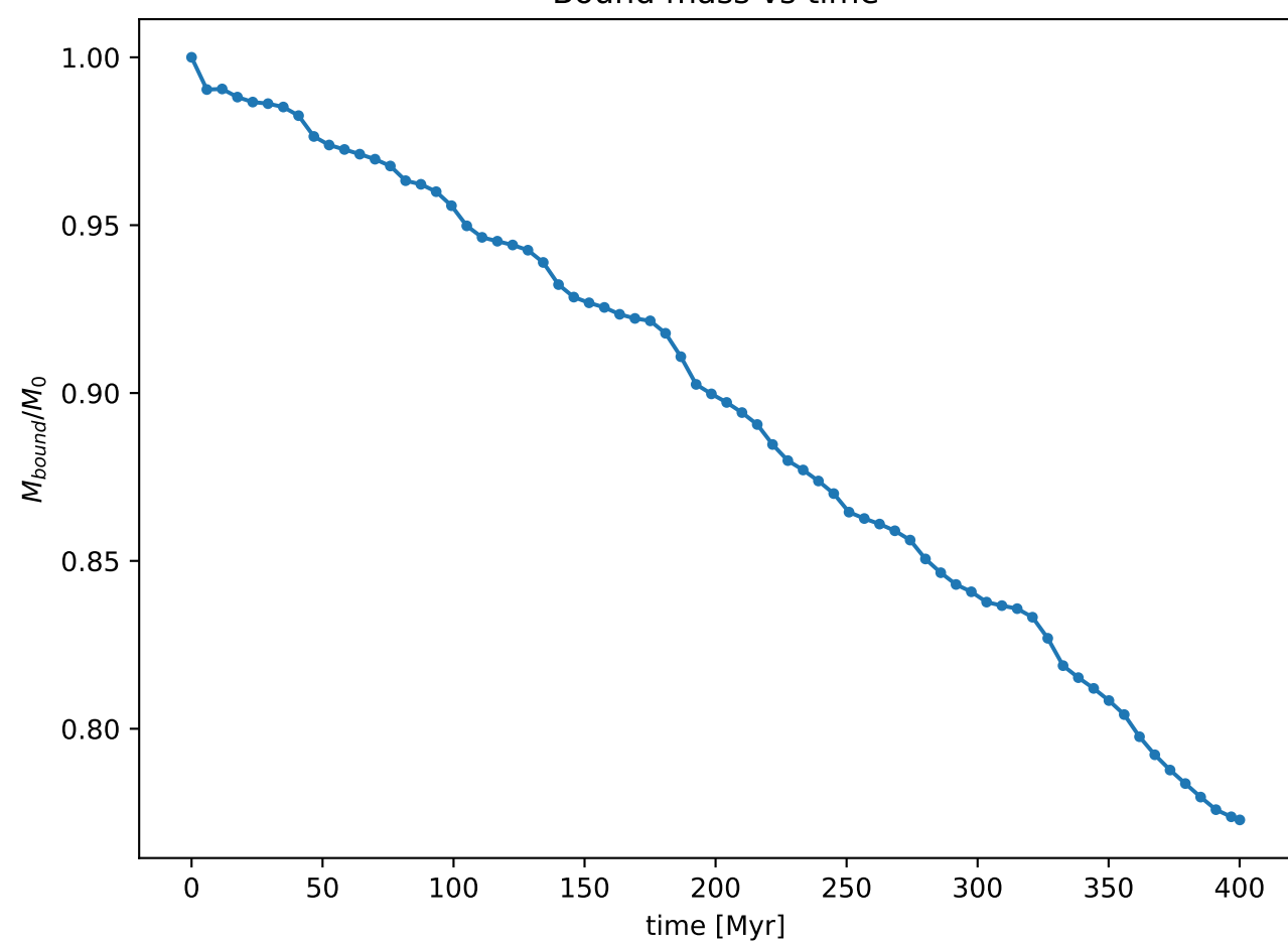
Bound mass vs time
