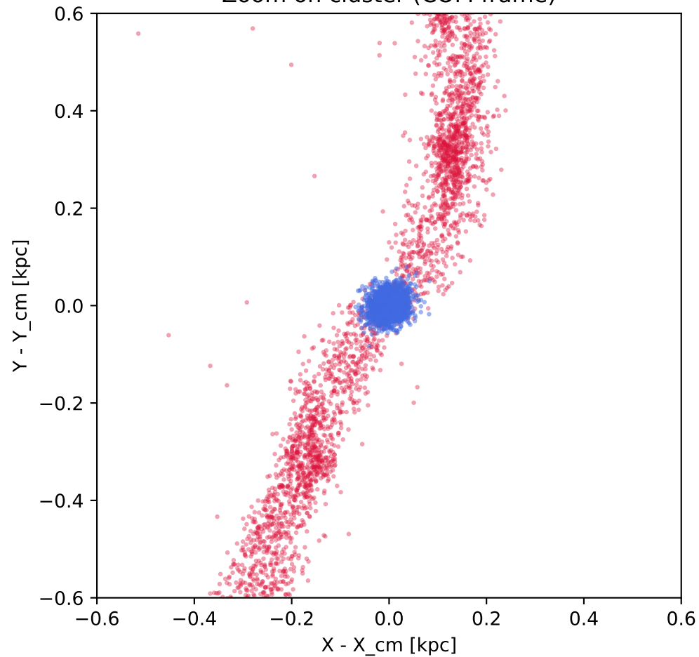
Zoom on cluster (COM frame)
