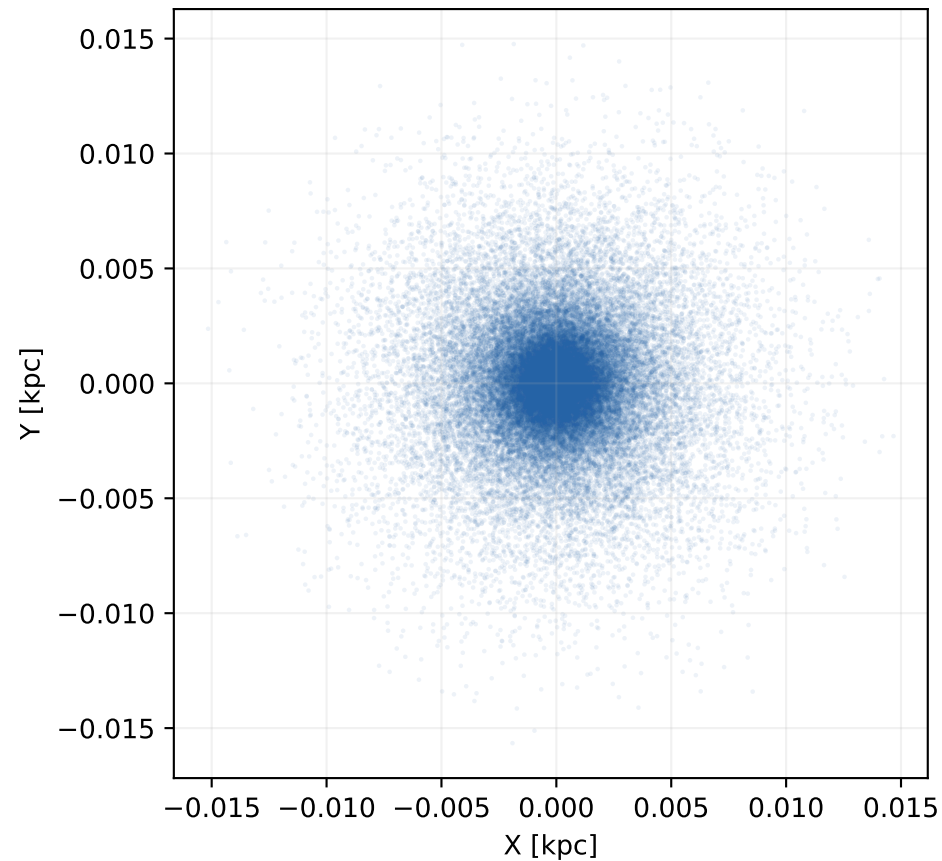
Initial compact King model
