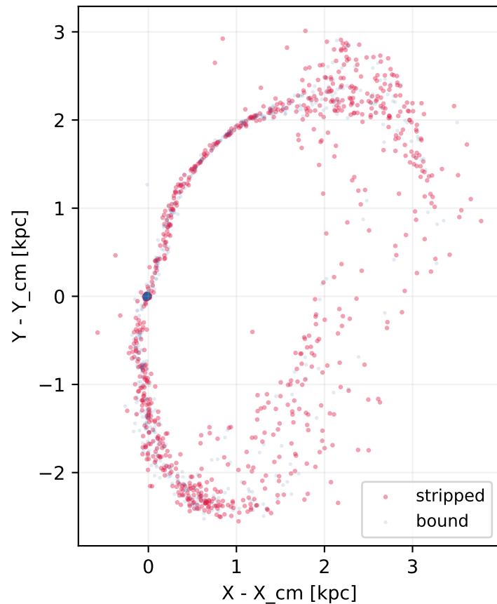
Final snapshot in remnant frame
