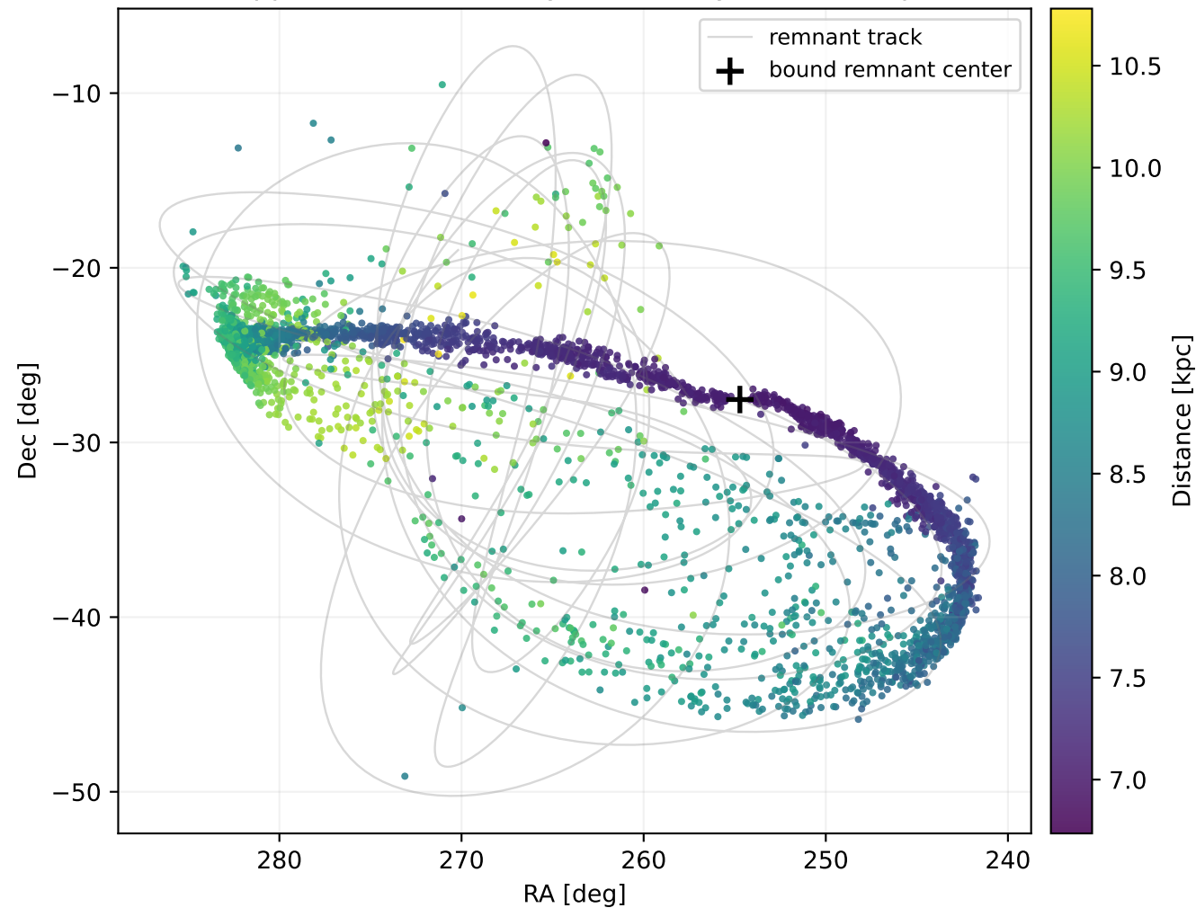
Stripped stars on the sky, colored by distance [kpc]
